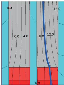
FIG. 5 Simulated temperature profile (THERM) at -5° C outside and 20° C inside for triple thermal insulation glazing 4/12/4/12/4 with U_g = 0.70 \text{ W/m}^2 \cdot \text{K} (left) and vacuum glazing 4 / 0.15 / 4 with U_g = 0.42 \text{ W/m}^2 \cdot \text{K} (right)
