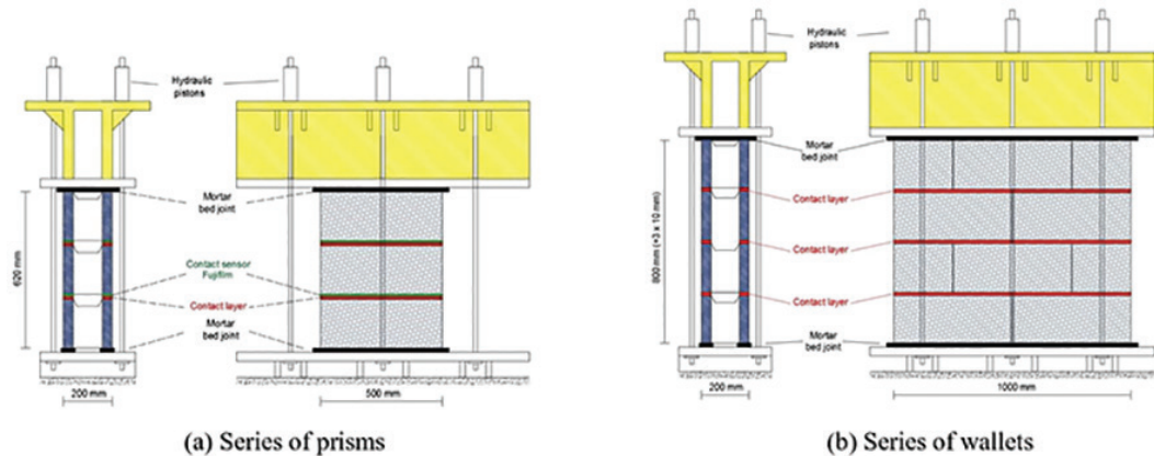
FIG. 3 Design of the experimental tests on (a) prisms and (b) masonry wallets (Gelen Gaël Chewe Ngapeya & Waldmann, 2020)
