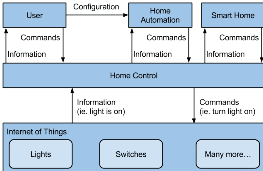
Figure 10.3: The HA landscape
