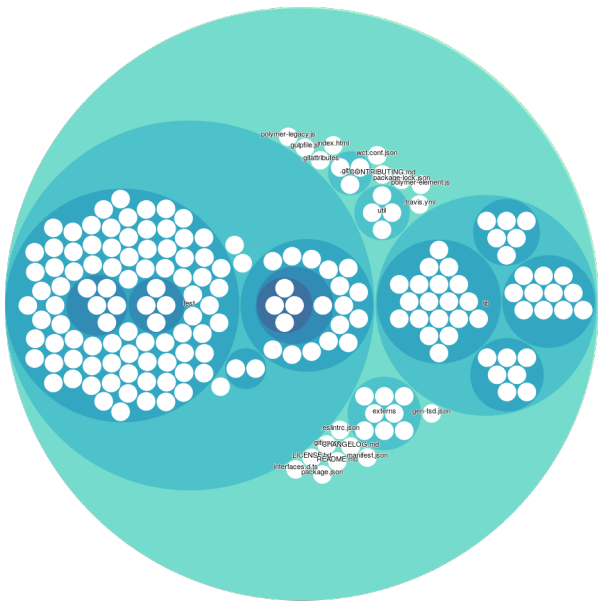
Figure 18.3: Source code file structure. The white circles are files. The names of the corresponding folders is displayed
