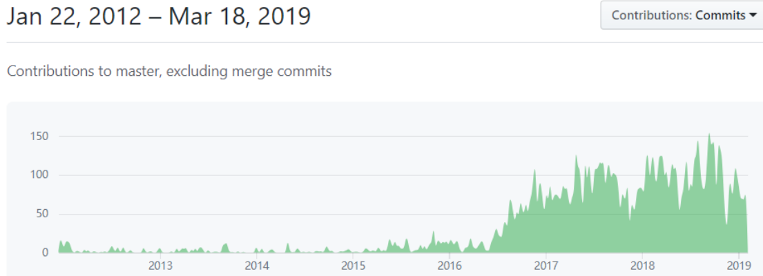
Figure 20.10: Contributions to master, excluding merge commits
