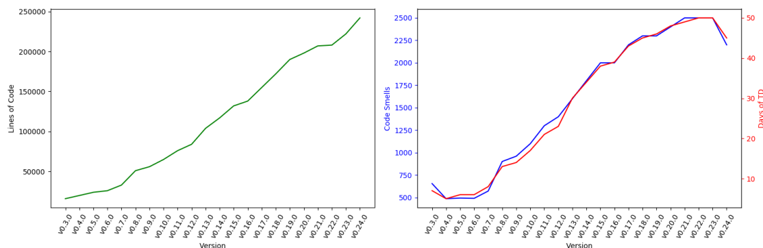
Figure 13: History of technical debt of the pandas project, excluding the HTML files.
