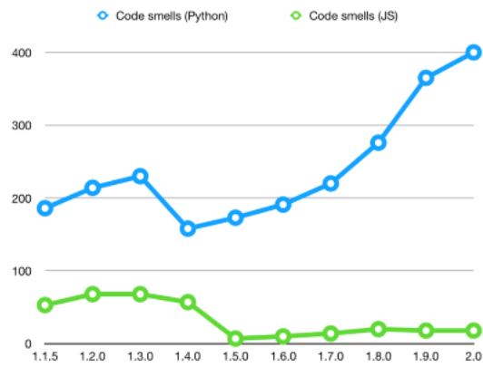
Figure 28.7: The progression of the number of code smells in the code base of Zulip
