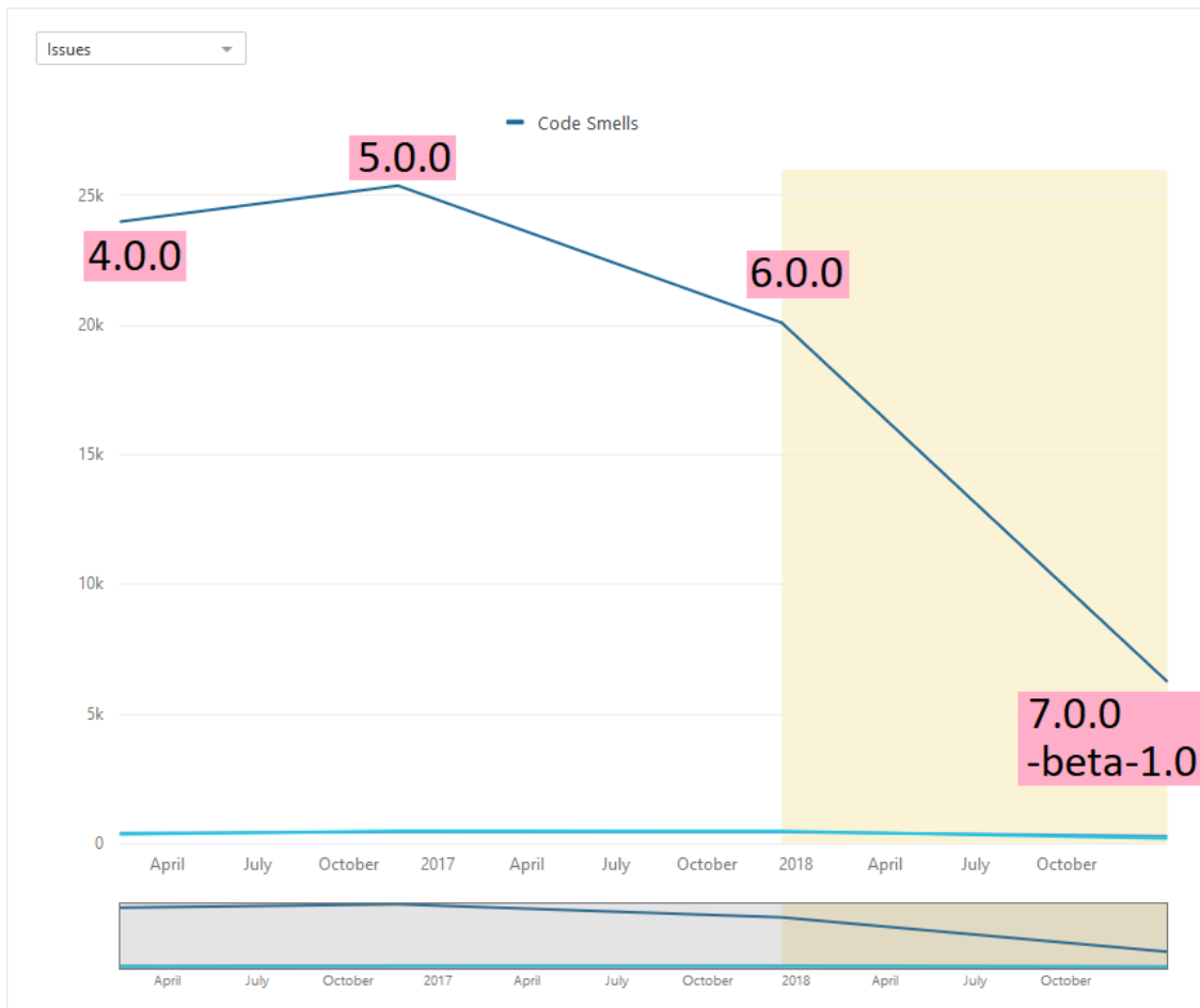
Figure 4.5: Evolution of number of code smells in Eclipse Che
