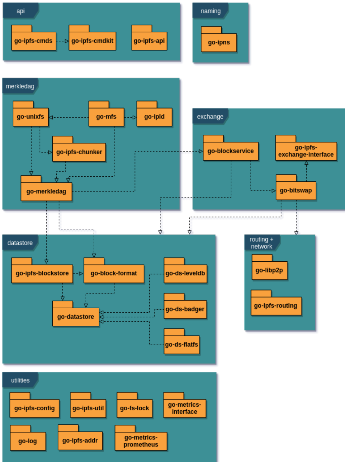
Figure 11.6: Package Diagram
