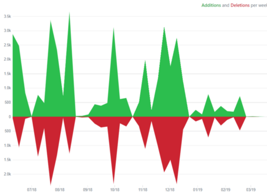
Figure 7.17: Code frequency
