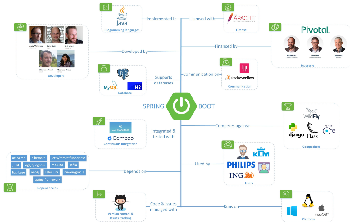
Figure 24.2: Context View
