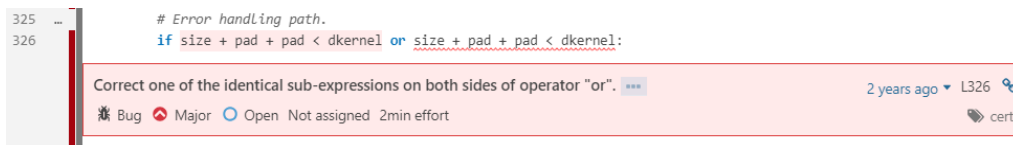
Figure 20.8: Specific bugs
