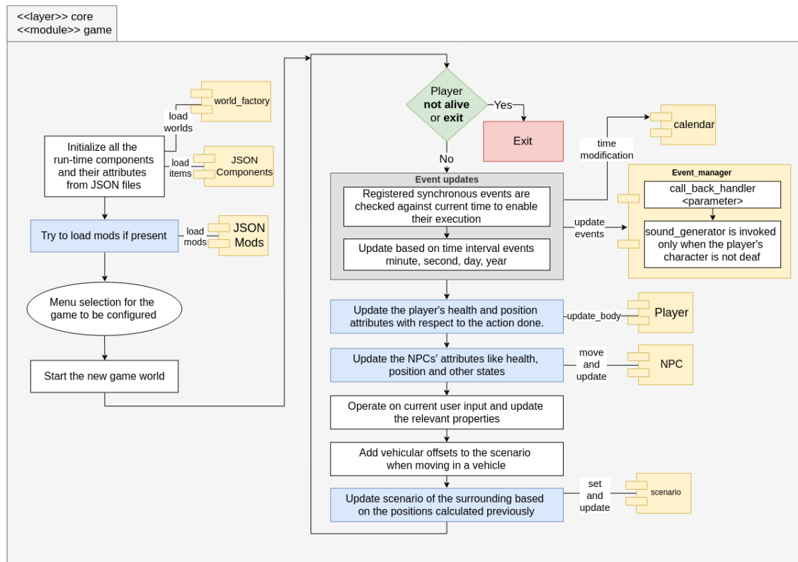
Figure 3.5: Context schema
