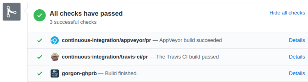
Figure 3.3: Continuous integration
