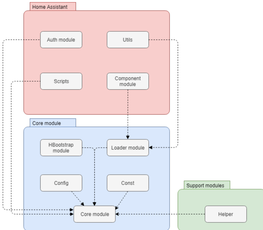
Figure 10: Module organization.
