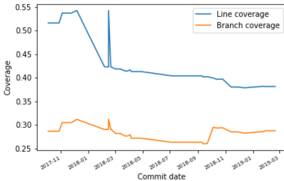
Figure 21.7: Coverage evolution
