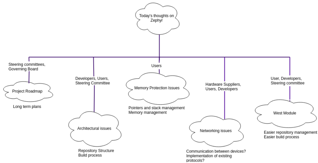
Figure 3 - Issue Clusters
