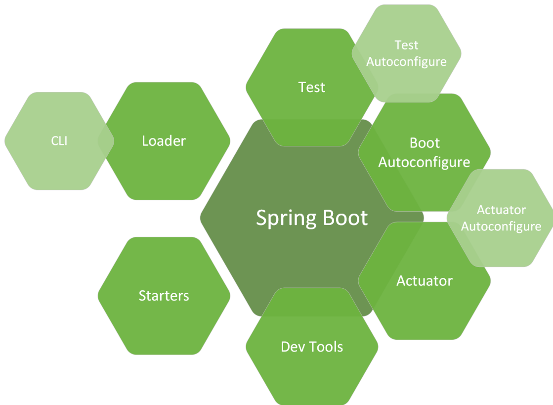
Figure 24.4: Module Structure
