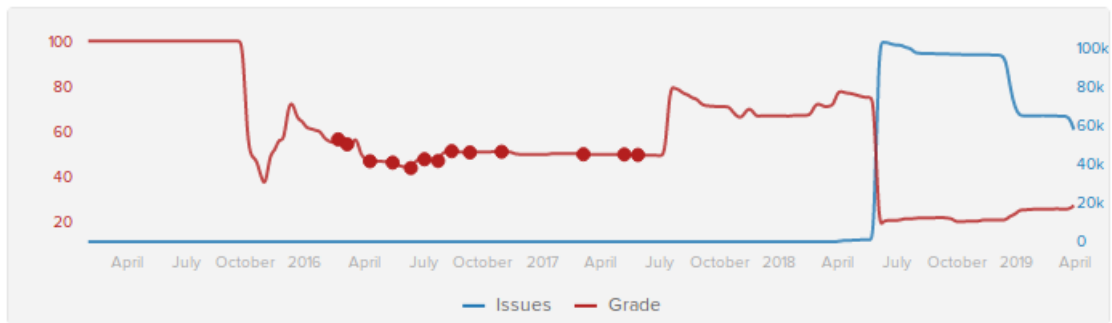
Figure 4.2. Code issue history.
