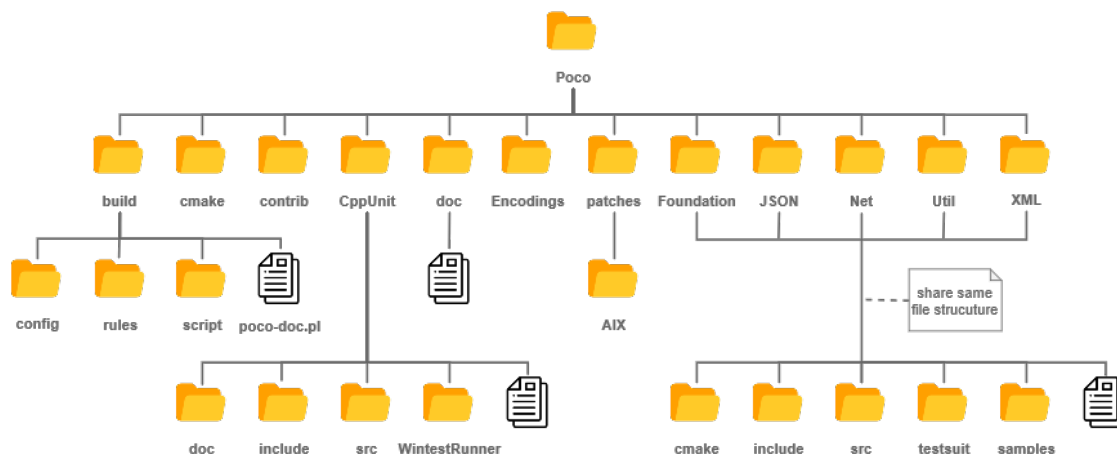
Figure 17.6: Codeline organisation of POCO
