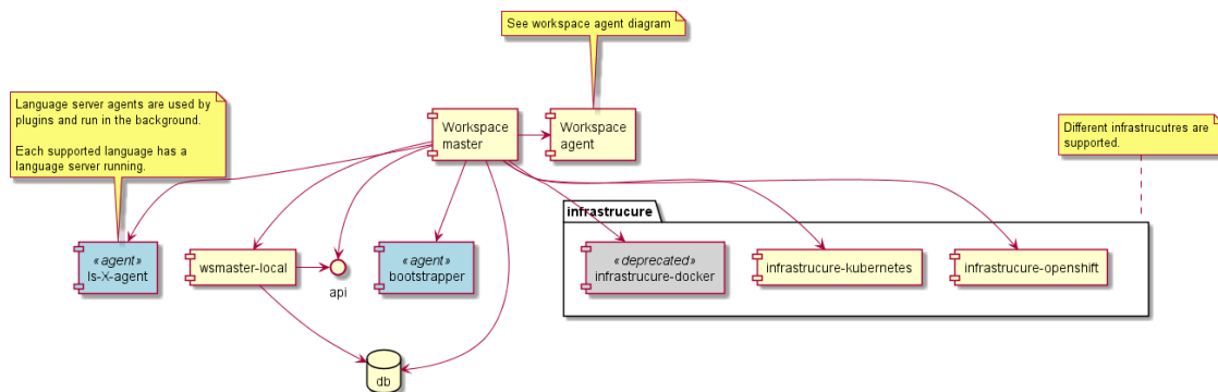
Figure 4.6: Top level module relationships
