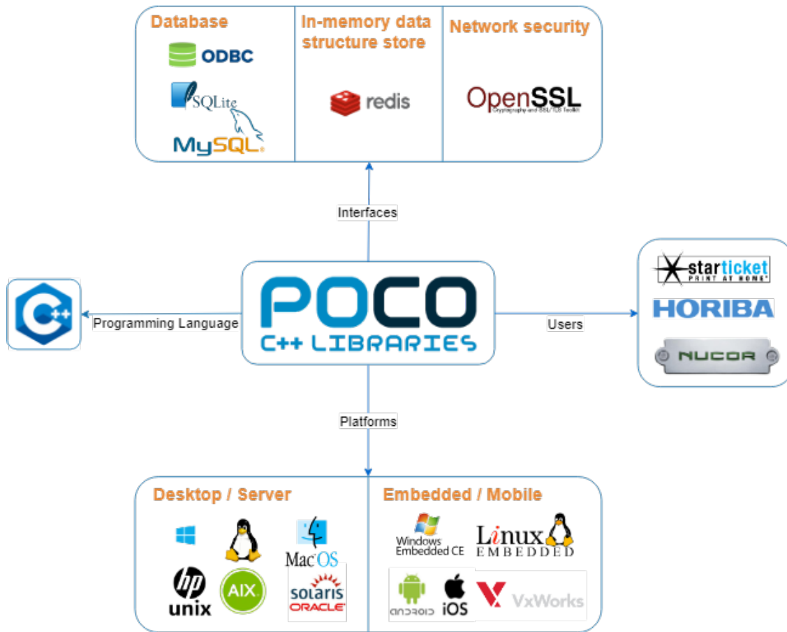
Figure 2 - Context view
