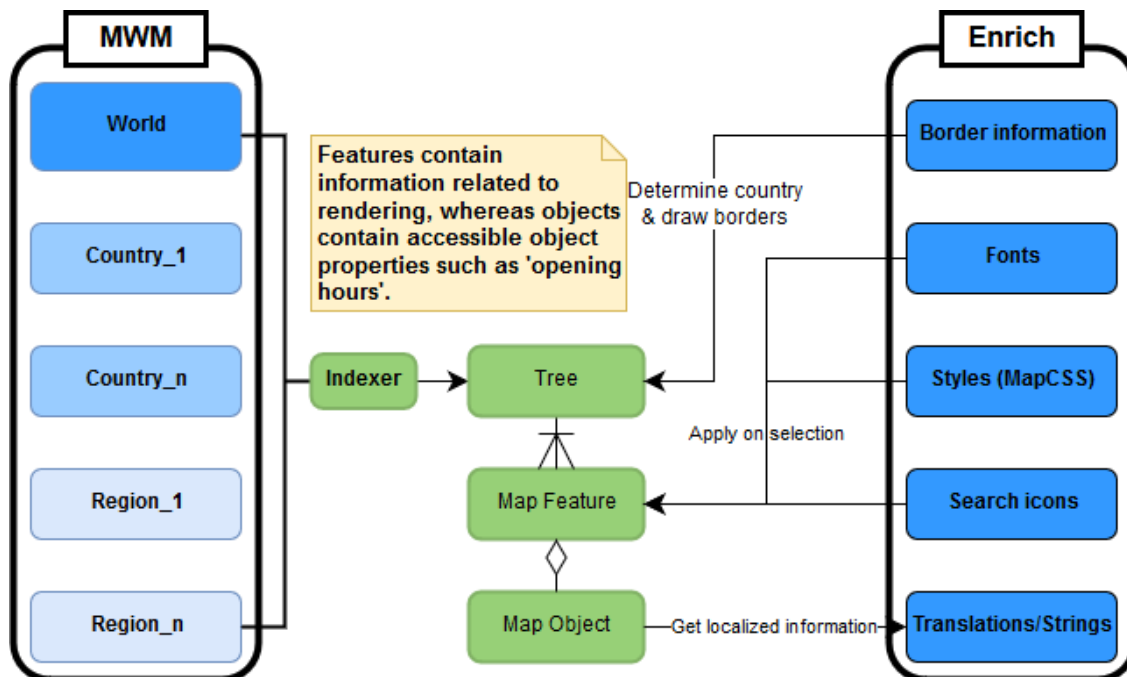
Figure 15.6: Figure 6: Information structure related to map files as static files and at runtime.
