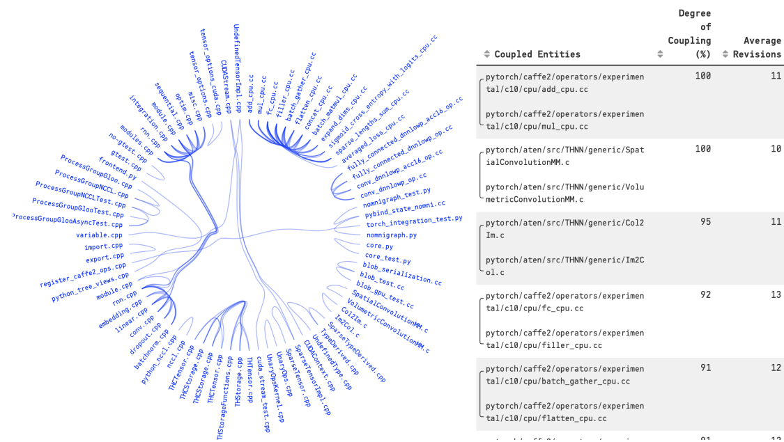
Figure 20.5: Temporal coupling
