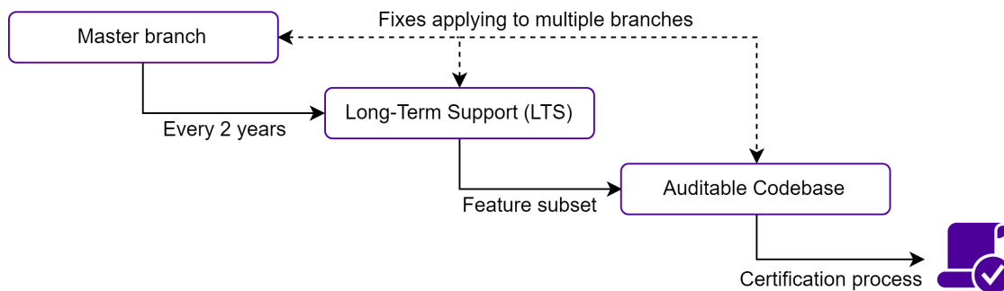
Figure 17 - Certification process
