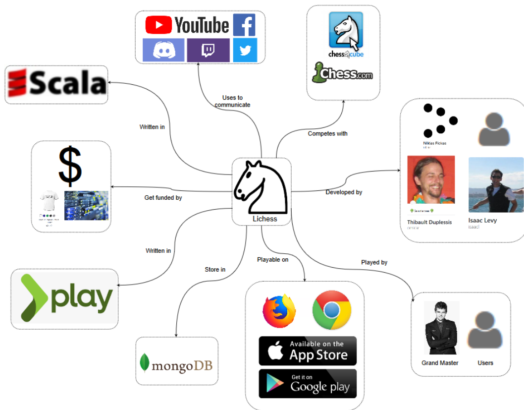
Figure 14.2: Context View
