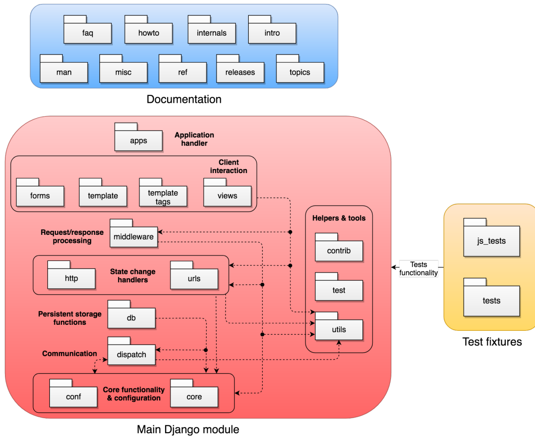
Figure 6.3: Django modules
