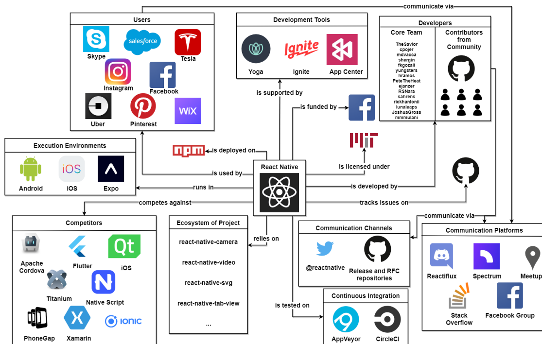
Figure 21.2: Context View
