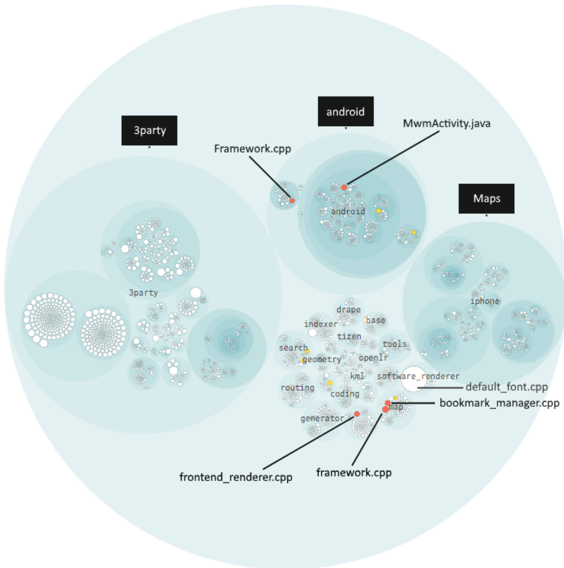
Figure 15.9: Figure 9: Refactoring candidates of MAPS.ME (from CodeScene)
