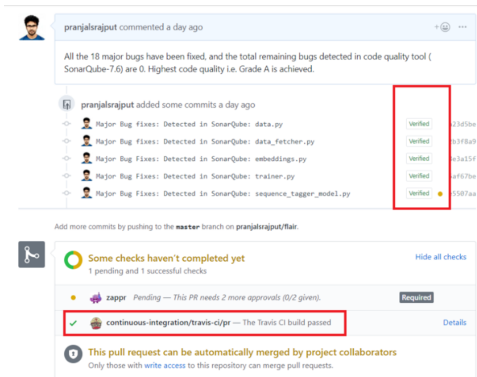
Figure 7.16: Pull request
