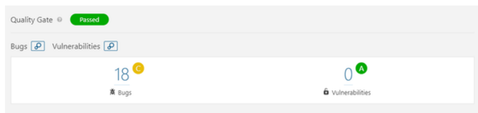
Figure 7.9: Detected bugs
