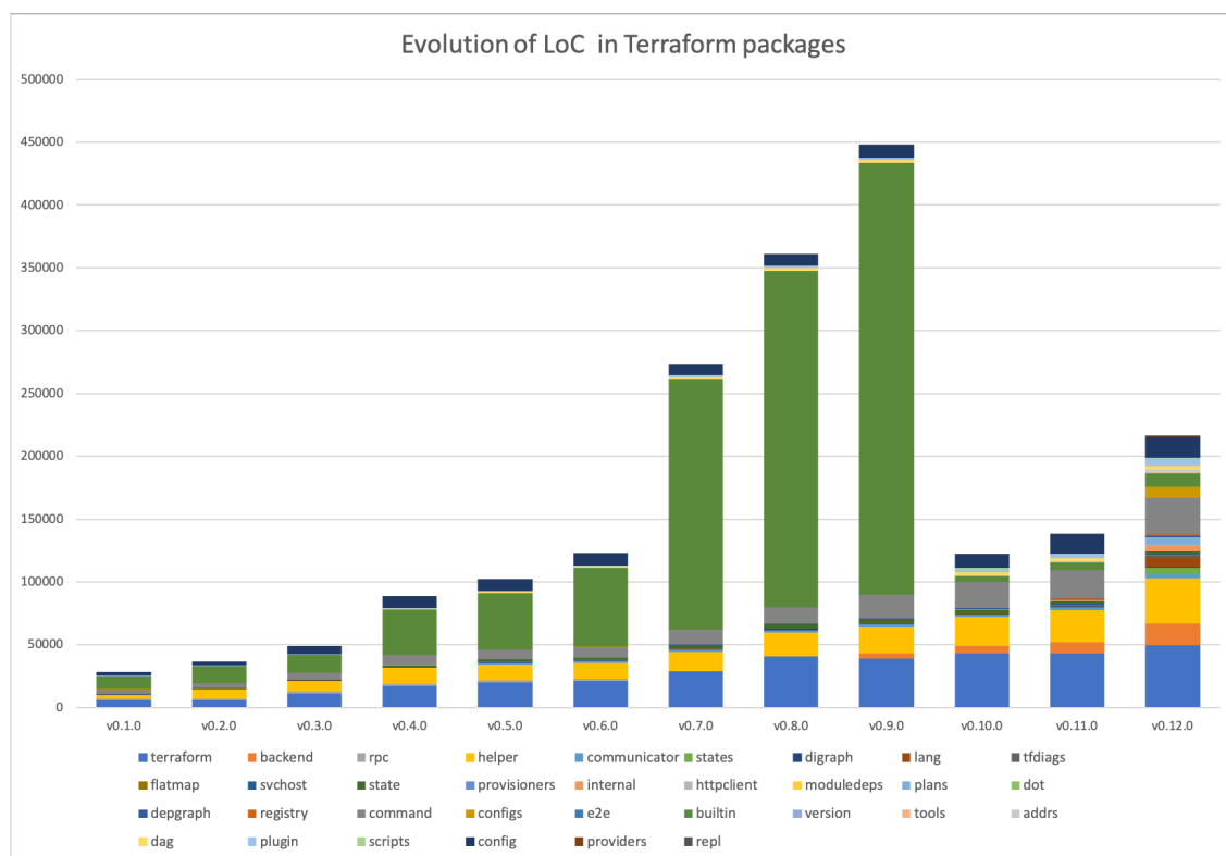
Figure 25.4: Evolution LoC
