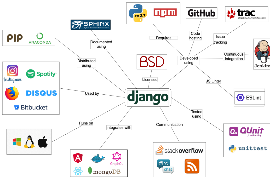
Figure 6.2: Context view
