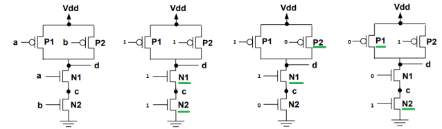
Fig. 4. (a) NAND schematic with (b) exhaustive PSA pattern {1,1} (c) exhaustive PSA pattern {1,0} (d) exhaustive PSA pattern {0,1} on its inputs a,b underlining the stressed MOSFETs [14]
