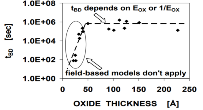
Fig. 6. Compiled TDDDB data for different oxide thickness [18]
