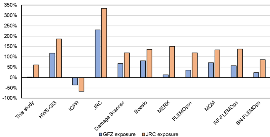
Fig. 7 Comparison between average modelled and reported losses during the 2010 coastal flood in France, for different damage models and exposure valuations
