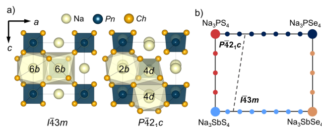
Figure 2. (a) Cubic (space group \bar{I}43m ) and tetragonal (space group P421c ) polymorph of the \text{Na}_3\text{PnCh}_4 structure family. (b) 2D substitution scheme of the investigated \text{Na}_3\text{PnCh}_4 structure at room temperature. Each dot represents a composition, where the incremental change of the cations per dot is 0.25 and for the anions is 0.5. The transition from the tetragonal to the cubic polymorph is indicated by the dotted line. For clarity: At room temperature, the phase transition occurs between the compounds \text{Na}_3\text{PS}_3\text{Se} and \text{Na}_3\text{PS}_{2.5}\text{Se}_{1.5} as well as between the compounds \text{Na}_3\text{SbS}_{3.5}\text{Se}_{0.5} and \text{Na}_3\text{SbS}_3\text{Se} .
