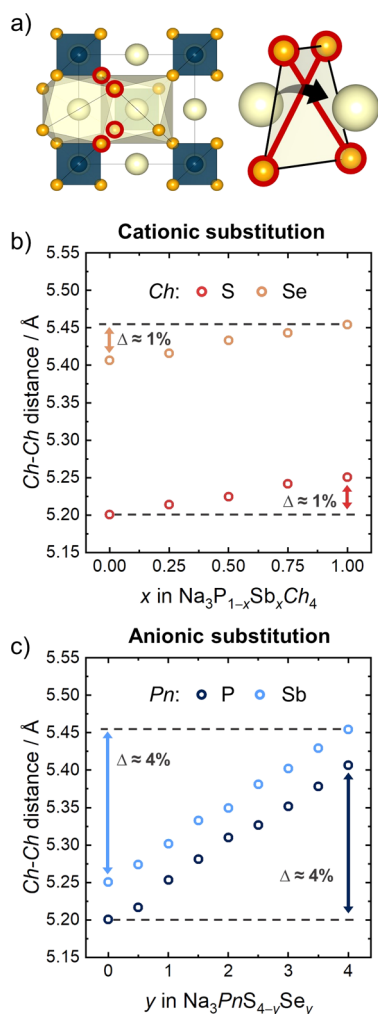
Figure 6. (a) Diffusion bottleneck in the \text{Na}_3\text{PnCh}_4 structure. The diffusion bottleneck consists of four Ch ions marked in red, which form a distorted square. The size of this square can be assessed from the square diagonals marked by red lines, which correspond to a crystallographic Ch–Ch distance. For the comparison of Ch–Ch distances in the cubic and tetragonal polymorph, an average over the four different Ch–Ch distances present in the tetragonal structure was calculated. The determined (averaged) Ch–Ch distances are shown in panel (b) for the cationic and panel (c) for the anionic substitution series. An increasing Ch–Ch distance is found upon the introduction of Sb and Se, with a more pronounced increase upon the anionic substitution.
