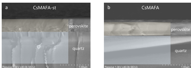
Figure 4A.22: Scanning electron microscopy (SEM) cross-section images of CsMAFA-st and CsMAFA with excess \text{PbI}_2 deposited on quartz. Light yellow and blue shades are guided by perovskite and quartz, respectively.
