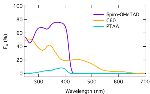
Figure 5A.3: Optical absorption spectra of Spiro-OMeTAD, C 60 , and PTAA layers deposited on quartz.
