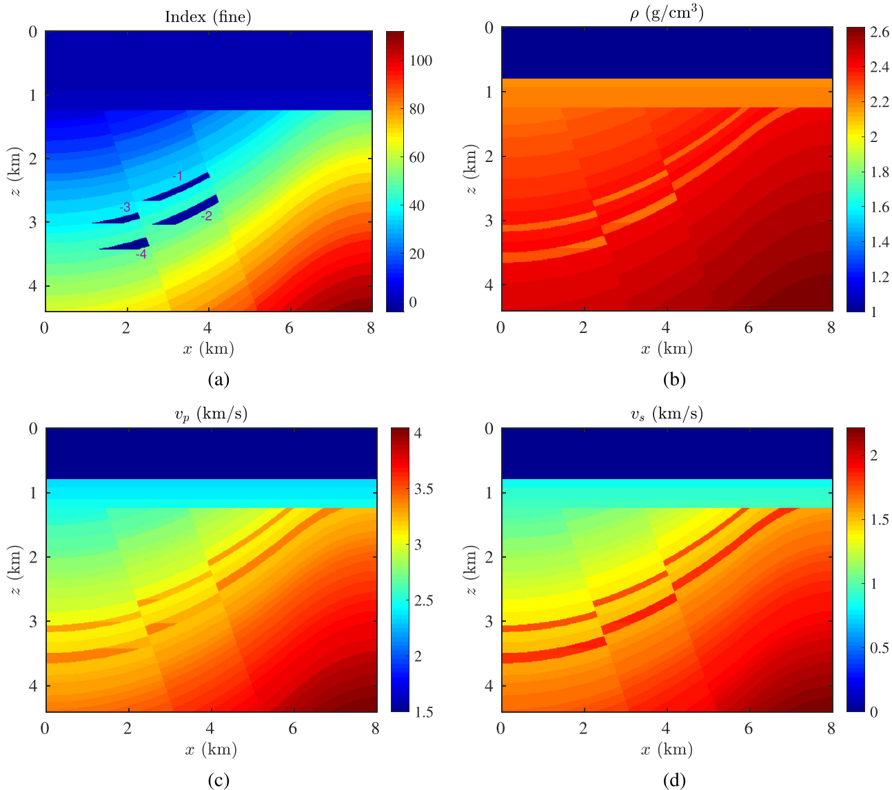
FIGURE 2 An index map (a) defines the piecewise constant values per layer for an isotropic elastic model with (b) density, (c) P- and (d) S-wave velocity. The negative indices correspond to four reservoirs.
