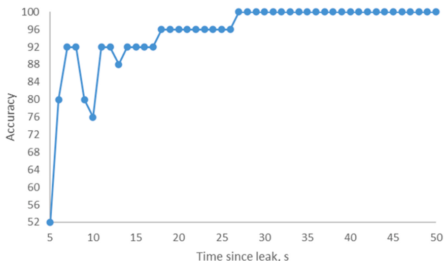
Fig. 6. Accuracy of gas leak classification using the same duration of training and testing data.
