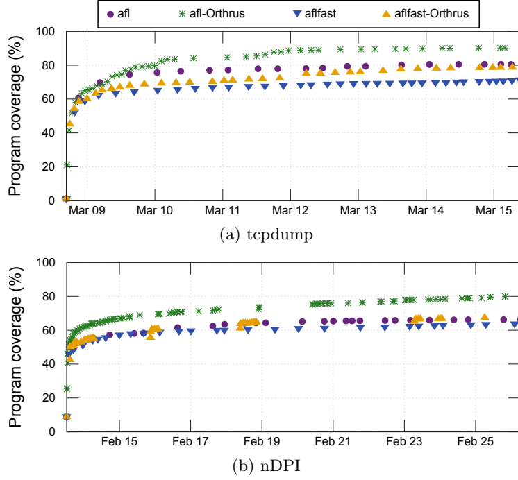
Fig. 3: Test coverage as a function of time for tcpdump 3a, and nDPI 3b, for different fuzzing configurations. Program coverage measurements were made only when there was a change in its magnitude.
