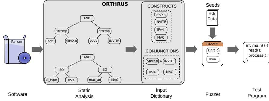
Fig. 1: Work-flow for program analysis guided fuzzing.
