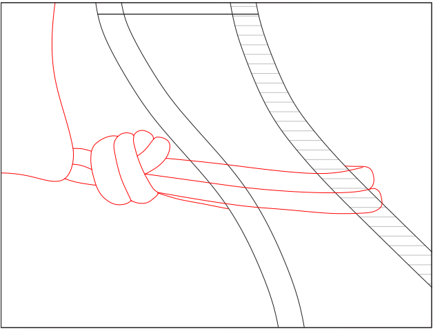
Bottom knot detail
