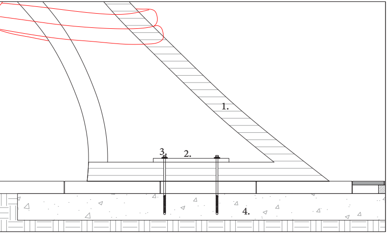
Base plate connection detail
