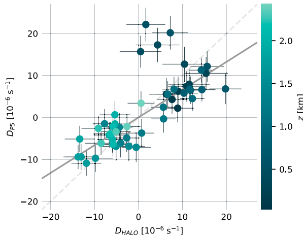
FIG. 4. Correlation between divergence profiles from HALO (RF11 C02) and P5 measurements on collocated flights for different heights (binned into bins of 50 m) (color scale) on 30 Mar 2022 obtained via regression method, correlation coefficient r = 0.734 and correlation fit D_{PS} = (0.662 \pm 0.008 \times D_{HALO} + (7.826 \times 10^{-7} \pm 6.55 \times 10^{-13}) \text{ s}^{-1}) (gray line), both excluding four outliers at 500 m (shaded).
