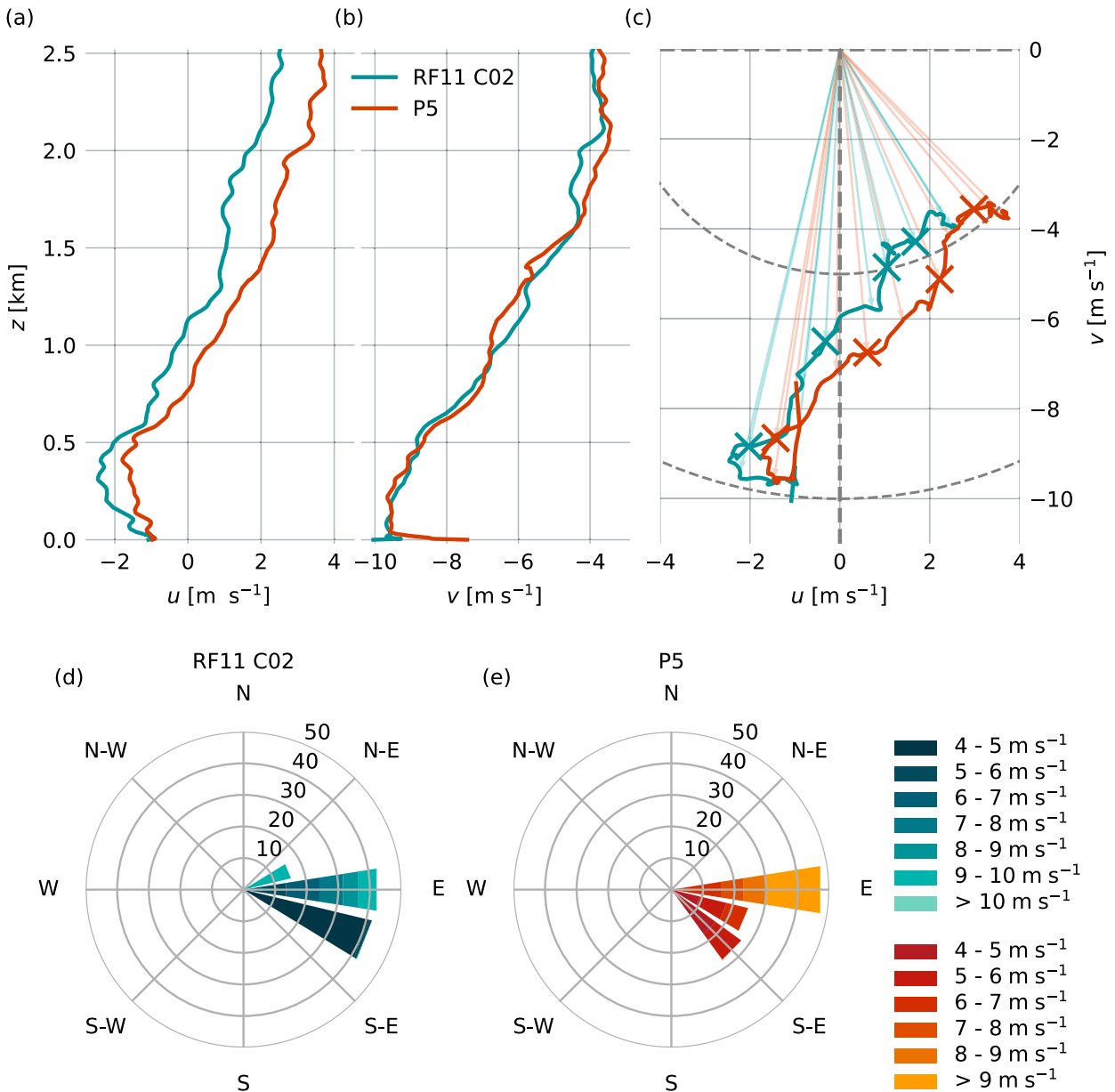
FIG. F1. Vertical profiles of horizontal wind velocities (a) u and (b) v and (c) hodograph for collocated flights RF11 C02 and P5 and wind rose plots for (d) RF11 C02 and (e) P5.
