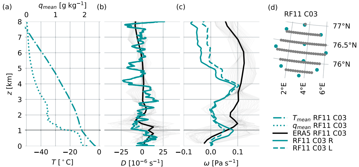
FIG. D5. (a) Vertical profiles of temperature T and specific humidity q , (b) vertical profiles of divergence D , and (c) pressure velocity \Omega at all grid points of ERA5 within the sampling area (light gray), averaged over all ERA5 grid points within the sampling area (black), and from dropsondes obtained with the regression method (blue) and line-integral method (blue, dashed), and (d) dropsonde locations of RF11 C03 and grid points of ERA5 (1200 UTC 30 Mar 2022) inside the sampling area.
