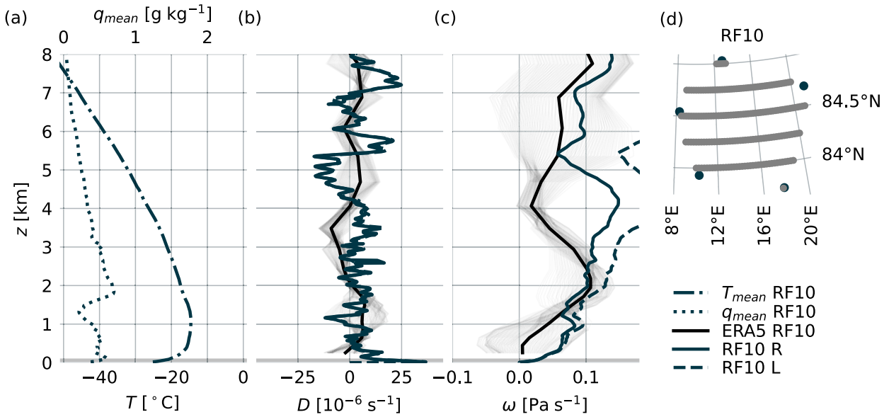
FIG. D2. (a) Vertical profiles of temperature T and specific humidity q , (b) vertical profiles of divergence D , and (c) pressure velocity \Omega at all grid points of ERA5 within the sampling area (light gray), averaged over all ERA5 grid points within the sampling area (black), and from dropsondes obtained with the regression method (blue) and line-integral method (blue, dashed), and (d) dropsonde locations of RF10 and grid points of ERA5 (1400 UTC 29 Mar 2022) inside the sampling area.
