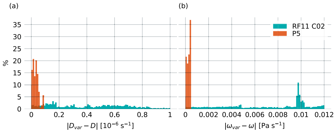
FIG. B1. Relative frequency distribution of the absolute differences in the (left) divergence and (right) pressure velocity profiles calculated with the line-integral method, when disregarding or accounting for potential pattern deformation with height ( D, \Omega and D_{var}, \Omega_{var} , respectively). For the RF11 C02 flight (blue), pattern deformation includes changes in both the circle radius and relative dropsonde distances; for P5 (red), only changes in the area enclosed by the flight track are considered.
