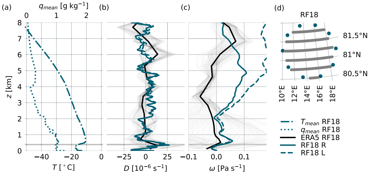
FIG. D6. (a) Vertical profiles of temperature T and specific humidity q , (b) vertical profiles of divergence D , and (c) pressure velocity \Omega at all grid points of ERA5 within the sampling area (light gray), averaged over all ERA5 grid points within the sampling area (black), and from dropsondes obtained with the regression method (blue) and line-integral method (blue, dashed), and (d) dropsonde locations of RF18 and grid points of ERA5 (1000 UTC 12 Apr 2022) inside the sampling area.
