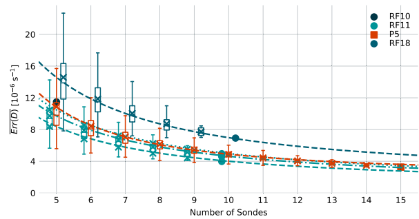
FIG. 5. Vertically averaged estimated error of divergence \overline{\text{Err}(D)} for all possible combinations of sondes N (minimum five sondes) from the regression method (boxplots, outliers not shown, RF11 and RF18 displaced for better visualization) and data from all circles of RF11 combined in one boxplot for better readability. Mean estimated error of all combinations x , estimated error for maximum number of sondes (bold marker), and power-law fit \Delta D = aN^{-b} + c for RF11 C01 (dotted), RF11 C02 (dashed), RF11 C03 (dash dotted), RF08, and RF18; see Table G1 in appendix G for fit parameters.
