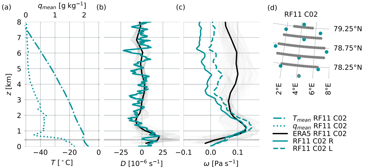
FIG. D4. (a) Vertical profiles of temperature T and specific humidity q , (b) vertical profiles of divergence D , and (c) pressure velocity \Omega at all grid points of ERA5 within the sampling area (light gray), averaged over all ERA5 grid points within the sampling area (black), and from dropsondes obtained with the regression method (blue) and line-integral method (blue, dashed), and (d) dropsonde locations of RF11 C02 and grid points of ERA5 (1100 UTC 30 Mar 2022) inside the sampling area.
