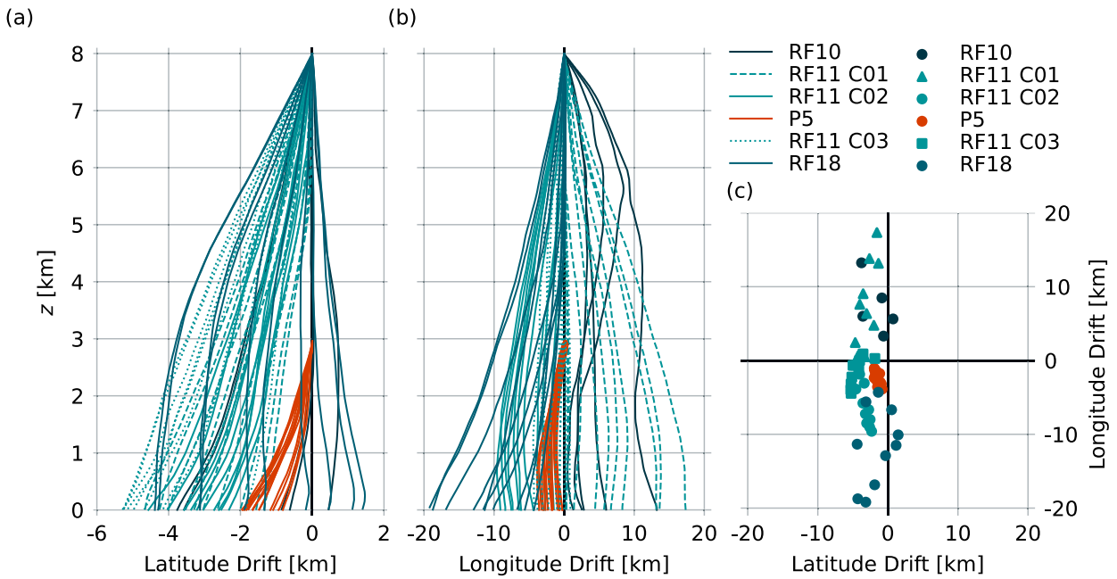
FIG. A1. Vertical profiles of horizontal displacement of dropsondes from the location of release at t_0 in (a) latitude \text{lat} - \text{lat}(t_0) , (b) longitude \text{lon} - \text{lon}(t_0) , and (c) maximum horizontal displacement.
