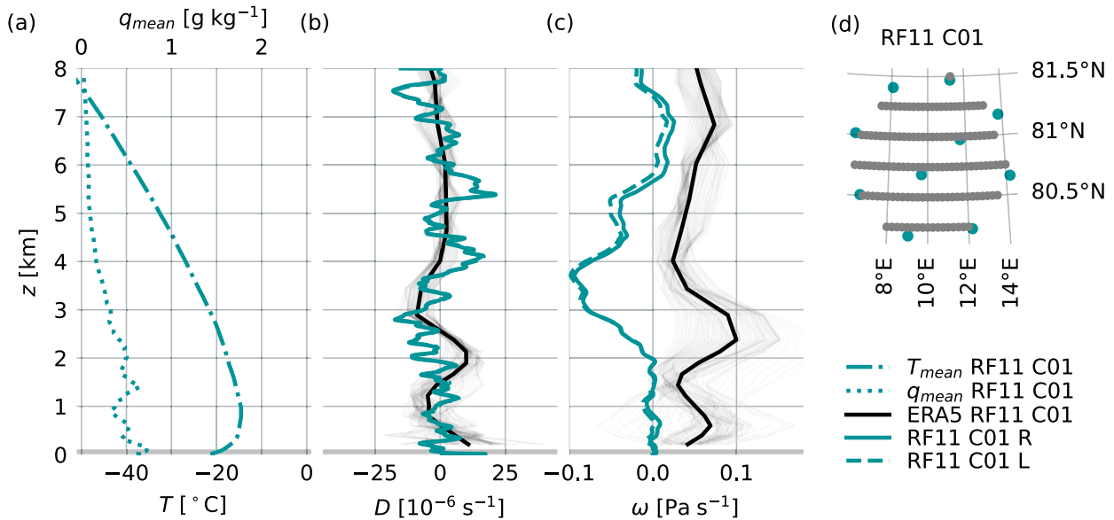
FIG. D3. (a) Vertical profiles of temperature T and specific humidity q , (b) vertical profiles of divergence D , and (c) pressure velocity \Omega at all grid points of ERA5 within the sampling area (light gray), averaged over all ERA5 grid points within the sampling area (black), and from dropsondes obtained with the regression method (blue) and line-integral method (blue, dashed), and (d) dropsonde locations of RF11 C01 and grid points of ERA5 (1000 UTC 30 Mar 2022) inside the sampling area.
