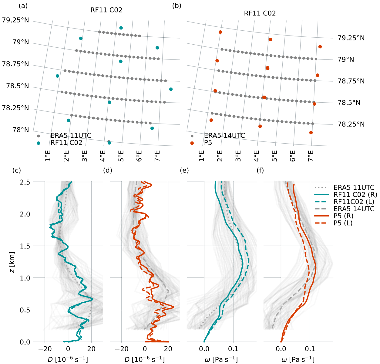
FIG. D1. Dropsonde locations of (a) RF11 C02 and (b) P5 and corresponding grid points of ERA5 [1100 UTC 30 Mar 2022 in (a) and 1400 UTC 30 Mar 2022 in (b)] inside the sampling area, vertical profiles of divergence D from (c) RF11 C02 and (d) P5 and pressure velocity \Omega from (e) RF11 C02 and (f) P5 at all grid points of ERA5 within the sampling area (light gray), averaged over all ERA5 grid points within the sampling area (black), and from dropsondes obtained with the regression method using all dropsondes [solid R (all)] and line-integral method (dashed L ).
