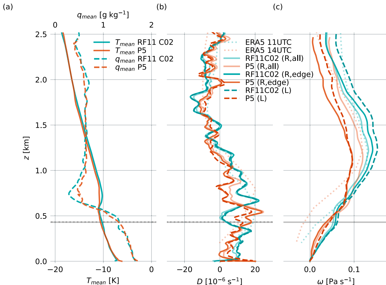
FIG. 3. Vertical profiles of the mean temperature T_{\text{mean}} and specific humidity q_{\text{mean}} , averaged over all dropsonde measurements deployed during each (a) flight, (b) mass divergence D , and (c) pressure velocity \omega obtained from dropsonde measurements from the collocated flight of HALO (RF11 C02) (blue) and P5 (red) aircraft on 30 Mar 2022. Regression method using all sondes R (all) (semitransparent), line-integral method (dashed), and regression method using only sondes which can be included in the line-integral method R (edge) (solid), mean divergence D , and pressure velocity \omega from ERA5 reanalysis (Hersbach et al. 2020) at 1100 UTC 30 Mar 2022 (approximate time of RF11 C02) and 1400 UTC (approximate time of P5), averaged over the flight areas (Figs. D1a,b), and height of the boundary layer h_{\text{BL}} = 0.43 km obtained from both flights (appendix E).
