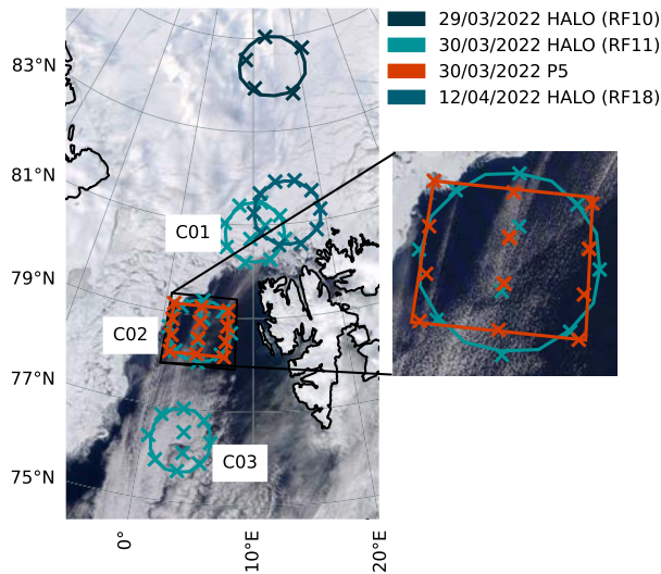
FIG. 1. HALO-(AC) 3 flight track patterns for three HALO flights (RF10, RF11, and RF18; blue) and P5 (red) with the locations of the dropsonde launches (x). Satellite image at the time of RF11 30 Mar 2022 from Terra MODIS (NASA 2022, Worldview Snapshots) in the background, adapted in modified form from Fig. 17a in Wendisch et al. (2024).
