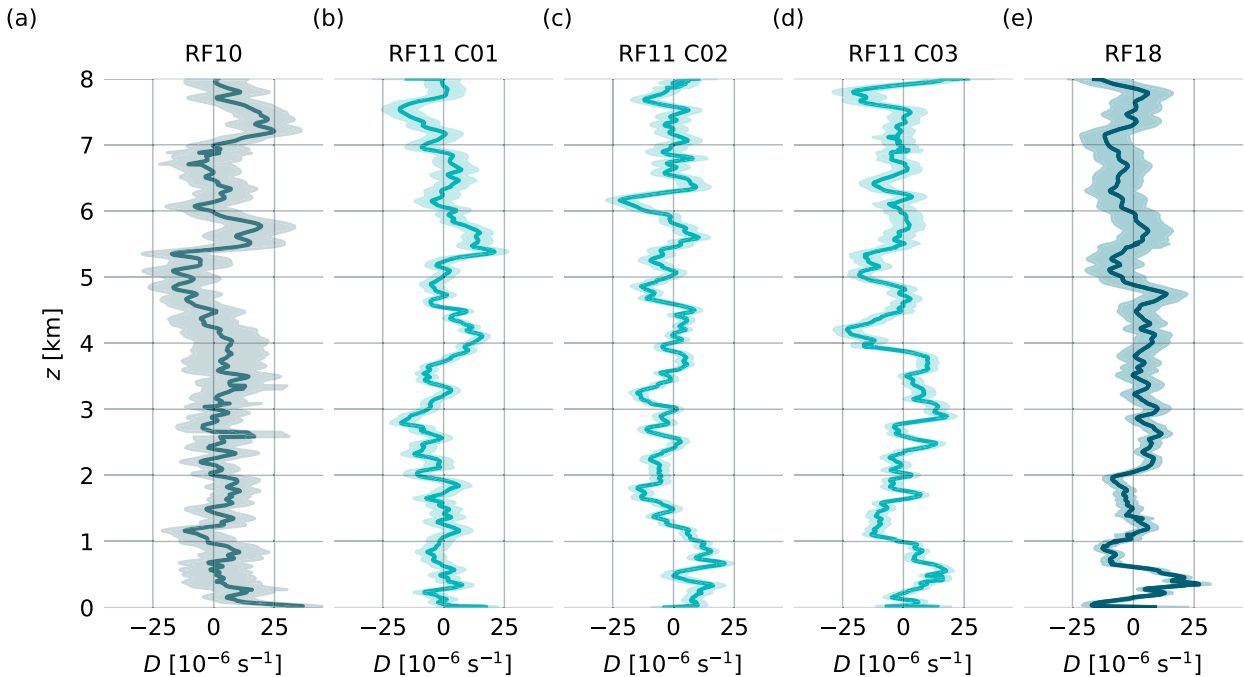
FIG. 2. Vertical profiles of wind divergence D obtained by the regression method from HALO pattern flights (a) RF10 (five sondes), (b) RF11 C01 (10 sondes), (c) RF11 C02 (10 sondes), (d) RF11 C03 (10 sondes), and (e) RF18 (10 sondes) with estimated error (shaded).
