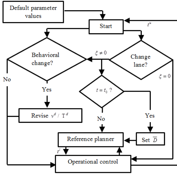
Fig. 3. Flowchart of tactical planning.
