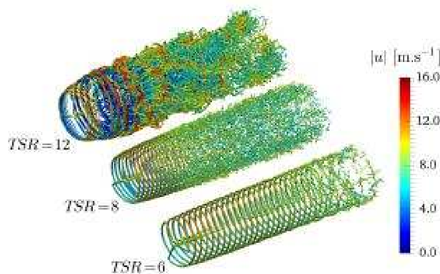
Figure 1: Iso-contour of Q-criterion Q=1 \text{ s}^{-2} colored by the norm of velocity for three Tip Speed Ratios.
