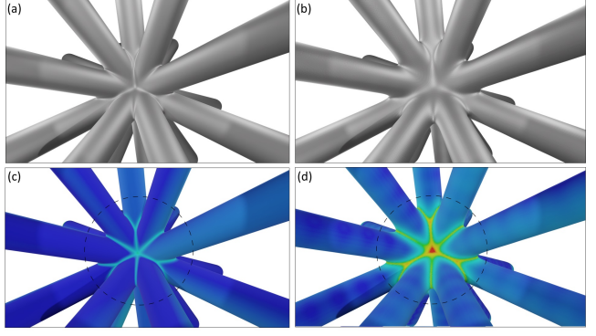
Fig. 3. Comparison of solids generated by our approach (a) and the Gaussian kernel (b) - both for the skeletons shown in Fig.1(a). It can clearly be observed that more over-blending artifacts are generated on the result of Gaussian kernel. The color maps in (c) and (d) are used to visualize the distance between implicit surfaces and the 'ideal' solid as the union of cylinders.
