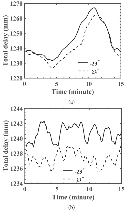
Fig. 11. Total slant delay time series for one pixel for two viewing angles ( -23^\circ and 23^\circ , angular difference 46^\circ ) for (a) the most changing pixel and (b) the least changing pixel in the domain. Note the differences in range on the vertical axis.
