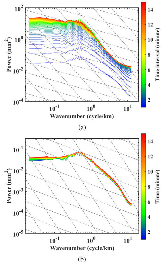
Fig. 9. One-dimensional power spectra synthetic interferogram combinations. (a) Unwrapped single master synthetic interferograms, i.e., cumulatively increasing delays over time. (b) Unwrapped daisy chain synthetic interferograms, i.e., only 10-s time differences. The dashed lines denote -8/3 and -2/3 power-law behavior. (a) Single master. (b) Daisy chain.
