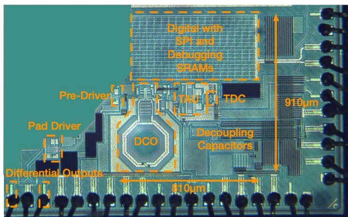
Figure 23.3.7: Die micrograph.
