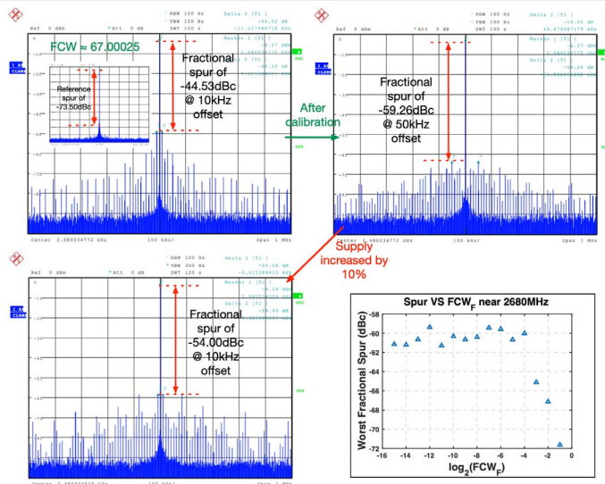
Figure 23.3.5: Measured reference and fractional spurs at a near-integer fractional-N channel (2680.04MHz), and the worst fractional spur versus the fractional part of the frequency-control word (FCW_F) near 2680MHz.
