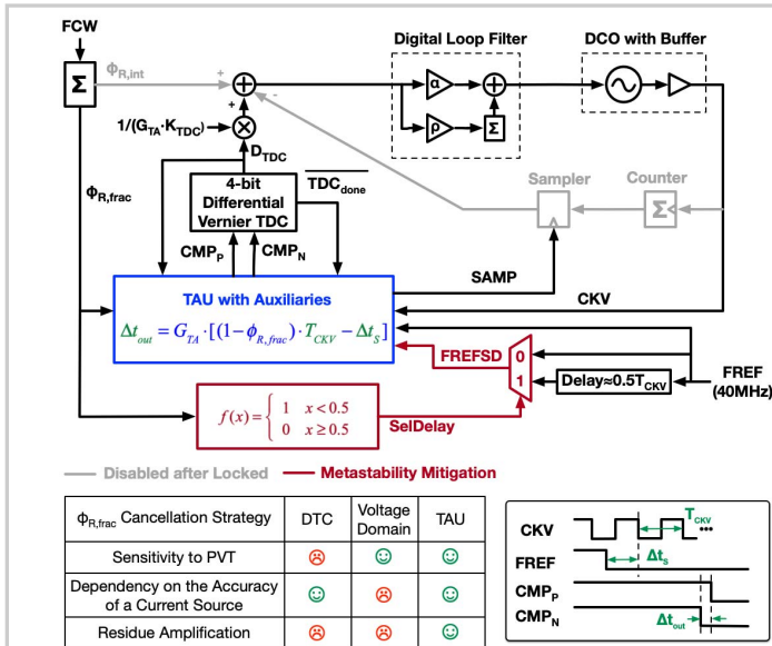
Figure 23.3.1: System overview of the proposed time-mode arithmetic-unit (TAU)-based PLL.
