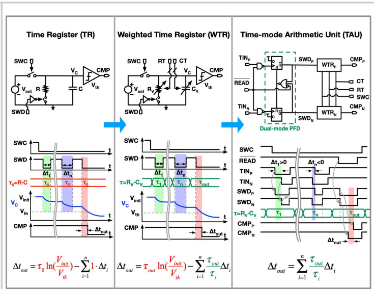
Figure 23.3.2: Conceptual implementation of the proposed TAU: evolution from the TR to the WTR and finally to the TAU.
