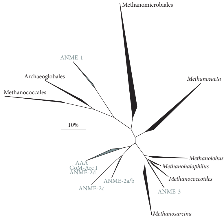
FIGURE 1: Phylogenetic tree of full length archaeal 16S rRNA sequences showing all methanotrophic clades so far described (grey) and other archaeal clades used in our domain based (meta)genome comparison (black). The tree was constructed with the ARB software package (version arb-6.0.1.rev12565) [49] using 2800 sequences from the SILVA SSURef NR 99 database (release 119.1) [50]. Trees were calculated by maximum likelihood analysis (RAxML, PHYML) and the ARB neighbor-joining method with terminal filtering and the Jukes-Cantor correction. Resulting trees were compared manually and a consensus tree was constructed. Sulfolobales as outgroup was removed after tree calculations. The scale bar represents the percentage of changes per nucleotide position.
