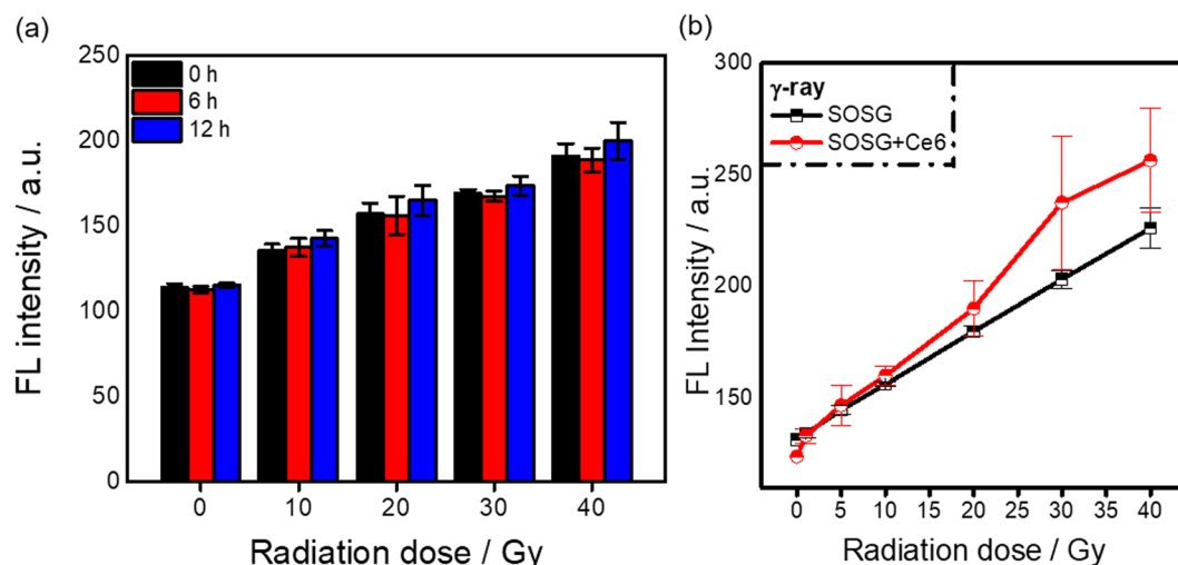
Figure 5. (a) Comparison of the fluorescence intensity at 529 nm for SOSG solutions (5 \mu M) at different time intervals after \gamma -ray irradiation of different radiation doses; (b) Comparison of the fluorescence intensity at 529 nm between pure SOSG solutions (5 \mu M) and SOSG solutions (5 \mu M) containing Ce6 (5 \mu M) ( \lambda_{\text{ex}} = 504 nm). (Error bars represent the standard deviation of at least 3 replicates).
