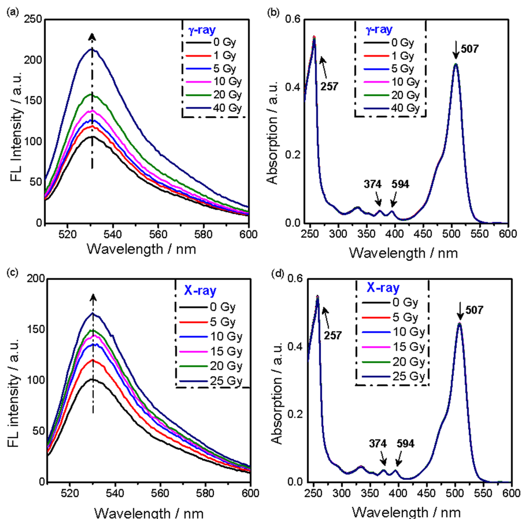
Figure 2. (a) Fluorescence spectra of SOSG solutions (5 μM) for varied radiation doses delivered by a ^{60}\text{Co} source ( \lambda_{\text{ex}} = 504 \text{ nm} ); (b) UV-vis absorption spectra of SOSG solutions (5 μM) for different radiation doses delivered by a ^{60}\text{Co} source; (c) Fluorescence spectra of SOSG solutions (5 μM) for different X-ray doses; (d) UV-vis absorption spectra of the SOSG solution (5 μM) for different X-ray doses.
