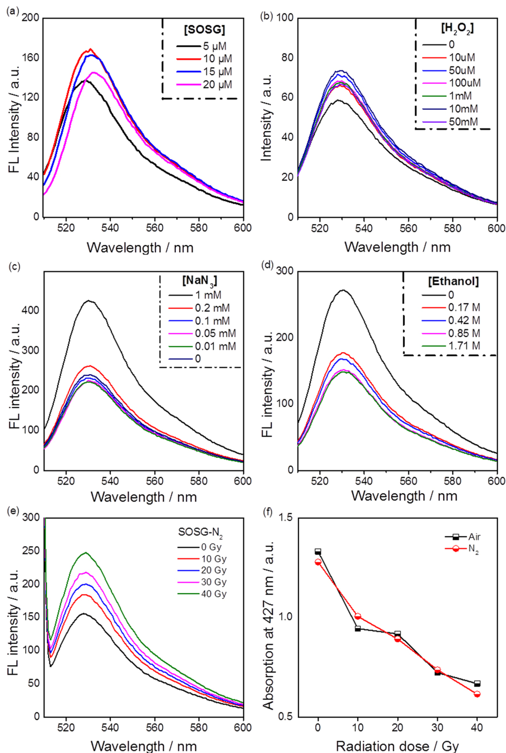
Figure 4. Fluorescence spectra ( \lambda_{\text{ex}} = 504 \text{ nm} ) of SOSG solutions (a) with varied SOSG concentrations, (b) reacted with H 2 O 2 solutions with varied concentrations, (c) reacted with NaN 3 solutions with different concentrations and (d) in the addition of varied amount of ethanol under 20 Gy radiation dose from a 60 Co source; Fluorescence spectra of SOSG solutions (5 μM) (e) saturated with N 2 for varied radiation doses delivered by a 60 Co source; (f) The FL intensity determined at 529 nm of air-saturated and N 2 -saturated SOSG solutions as function of radiation dose.
