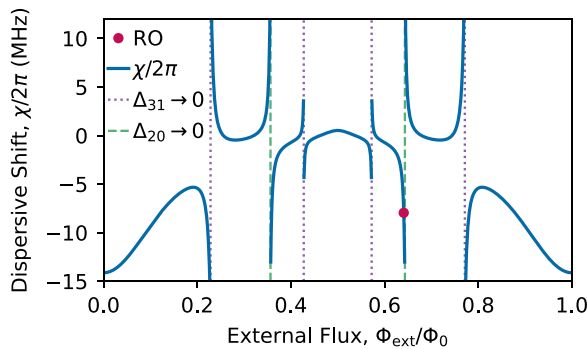
FIG. 3. The dispersive shift as a function of the external flux, where E_J/2\pi = 4.75 \text{ GHz} , E_C/2\pi = 1.25 \text{ GHz} , and E_L/2\pi = 1.5 \text{ GHz} . The targeted-readout (RO) point is marked with a red circle, the blue curve shows \chi/2\pi , and the dashed and dotted vertical asymptotes denote where a certain qubit transition, |i\rangle \leftrightarrow |j\rangle , and the resonator are on resonance, denoted by \Delta_{ij} \rightarrow 0 in the legend.
