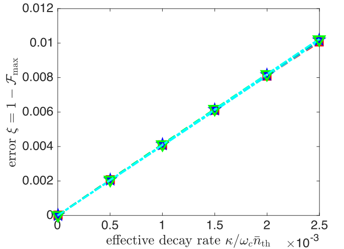
FIG. 15. Error as a function of the effective rethermalization rate \kappa \bar{n}_{\text{th}} for g/\omega_c = \frac{1}{16} (red squares), g/\omega_c = 1/(8\sqrt{2}) (blue stars) and g/\omega_c = \frac{1}{8} (green triangles), and k_B T/\omega_c = 2 ( \bar{n}_{\text{th}} \approx 1.54 ), within the relevant small-error regime ( \kappa_{\text{eff}}/g_{\text{eff}} \ll 1 ). The dashed-dotted lines in cyan refer to linear fits, demonstrating a linear error scaling in the small error regime ( \kappa_{\text{eff}}/g_{\text{eff}} \ll 1 ), which is independent of \mu = g/\omega_c . Accordingly, the error is larger for higher temperatures, but all temperature-related effects are approximately captured by the thermal occupation number \bar{n}_{\text{th}} . Other numerical parameters: \Gamma = 0 and \omega_q = 0 .
