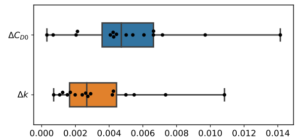
Figure 7. Absolute difference of drag polar between BADA (version 3.12) and model derived in this paper under clean configuration. (Note: A359, B789, E75L, and E195 are not presented in BADA model)
