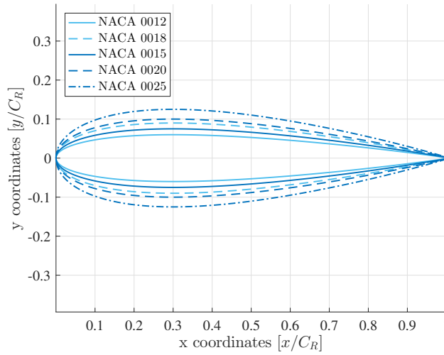
Figure 1: Tested NACA profiles.
