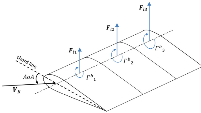
Fig. 5. The blade model of Kutta-Joukowski lift theorem and blade element theory.
