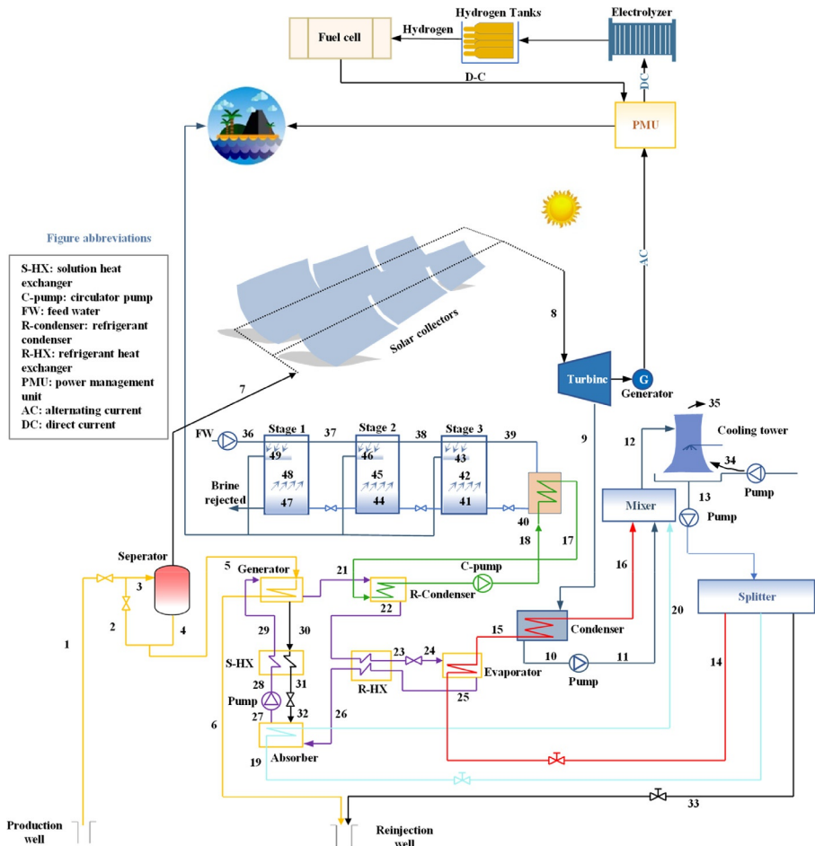
Fig. 4 A schematic diagram on an absorption refrigeration and solar-integrated geothermal power system with hydrogen storage.
