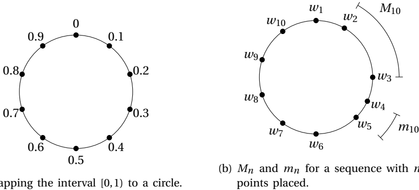
Figure 3.2.: How to map the circle to the interval [0, 1) , and how to measure M_n and m_n .
