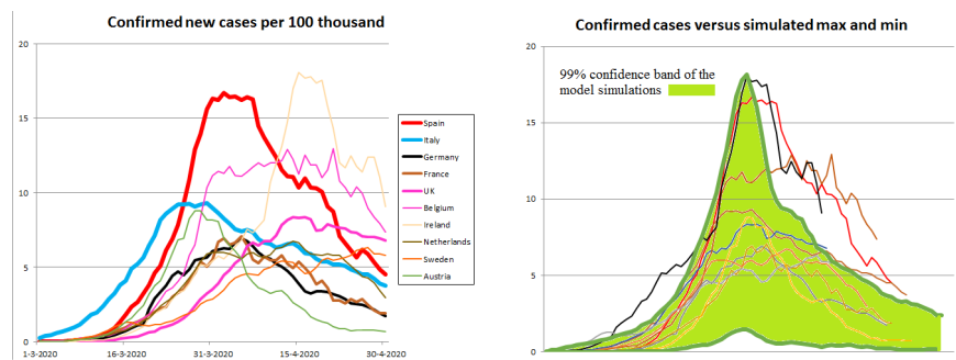
Figure 4.6.: A comparison of the daily number of officially confirmed new cases in ten EU countries during March and April 2020. The numbers are averaged over six days. In the right-hand figure, this data is adjusted so that the peak of the number of cases occurs after 50 days. This is compared to the 99% confidence band of a model computation with r = 0.055 pre-lockdown and r = 0.0075 during lockdown. Not all countries fit in the confidence band because their waves plateaued, while our model shows a sharp peak. The increase and decrease of the wave in our model does match the data.
