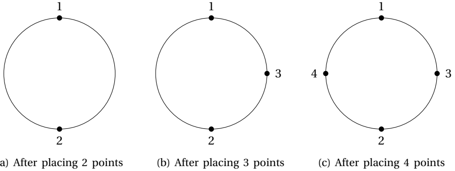
Figure 2.1.: An example of placing 4 points on a circle. The points are perfectly distributed over the circle when 2 points are placed and when 4 points are placed, but are not when 3 points are placed.
