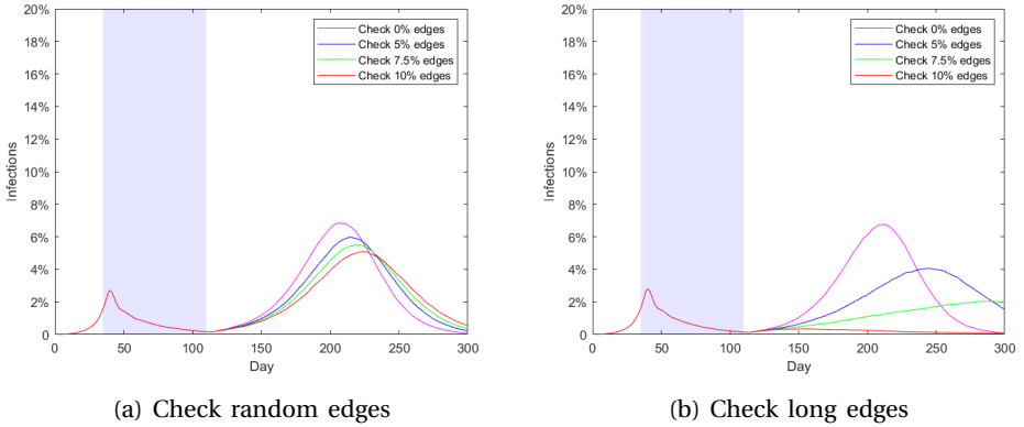
Figure 4.9.: Peak reduction with baseline r = 0.02 and some edges checked
