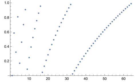
Figure 3.5.: The locations of the first points of the De Bruijn-Erdős sequence.
