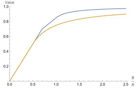
(b) \phi_i and \phi_i^\dagger for u_i = \frac{7}{10}
