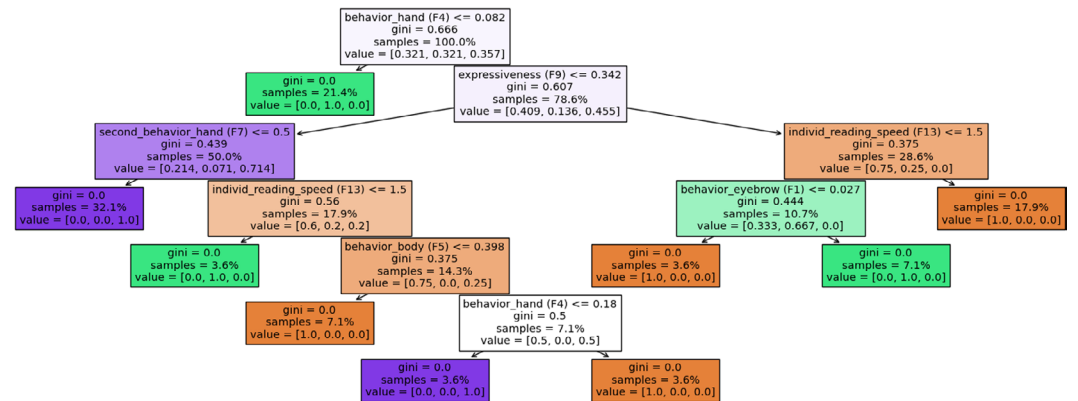
FIGURE B1 A plot tree to explain the model built upon the decision tree for predicting the unsupervised k-means clusters.
