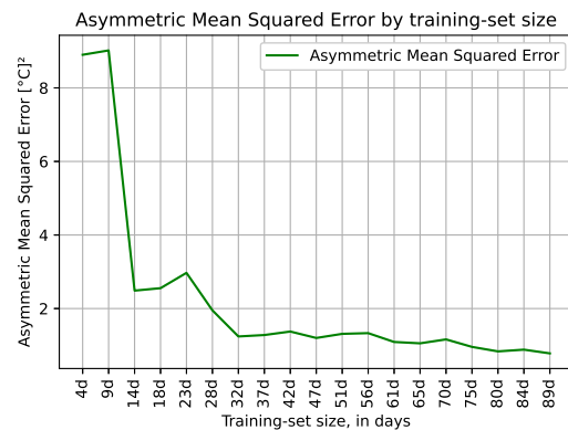
Figure 7. Variation of the errormetrics by increasing the data size used for the training phase. (a) represents the Mean Squared Error, (b) the Root Mean Squared Error and (c) the Asymmetric Mean Squared Error, defined in Section 3.3. On the x -axis, the number of days of data considered for the training. One month is sufficient to build a robust model, while more time brings no significant improvement.
