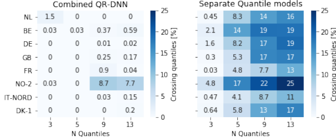
Fig. 5. Percentage of crossing quantiles per amount of quantiles included in the forecast, for both the QR-DNN and the separate quantile forecasts.
