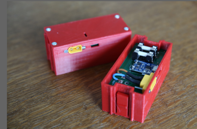
6.40. Custom battery PCB with charge/protection circuit and a fuse for each lithium cell.
