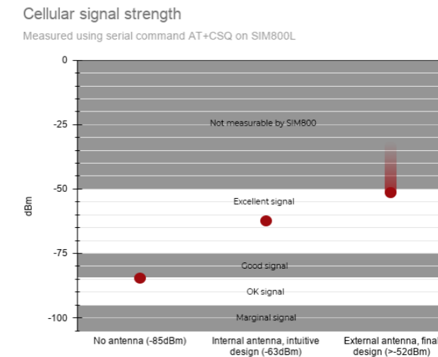
6.31. Signal strengths measured with different cellular antenna's
