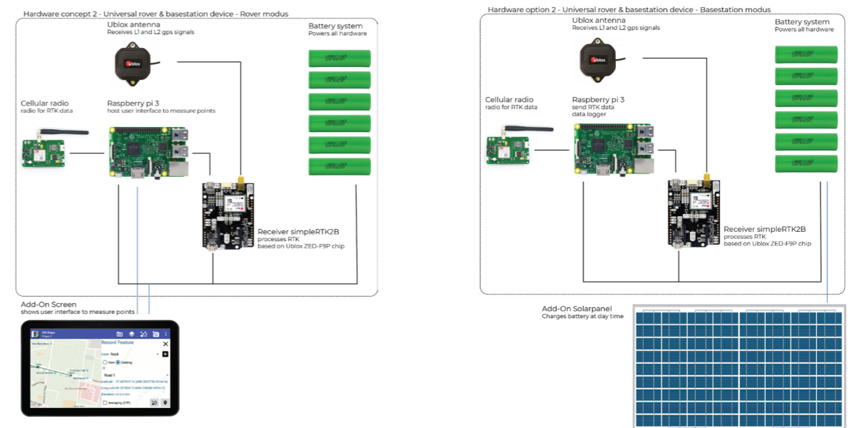
6.3. Hardware concept2. One universal device Left: Universal device used as rover with an add-on screen Right: Universal device used as base with a solar panel.
