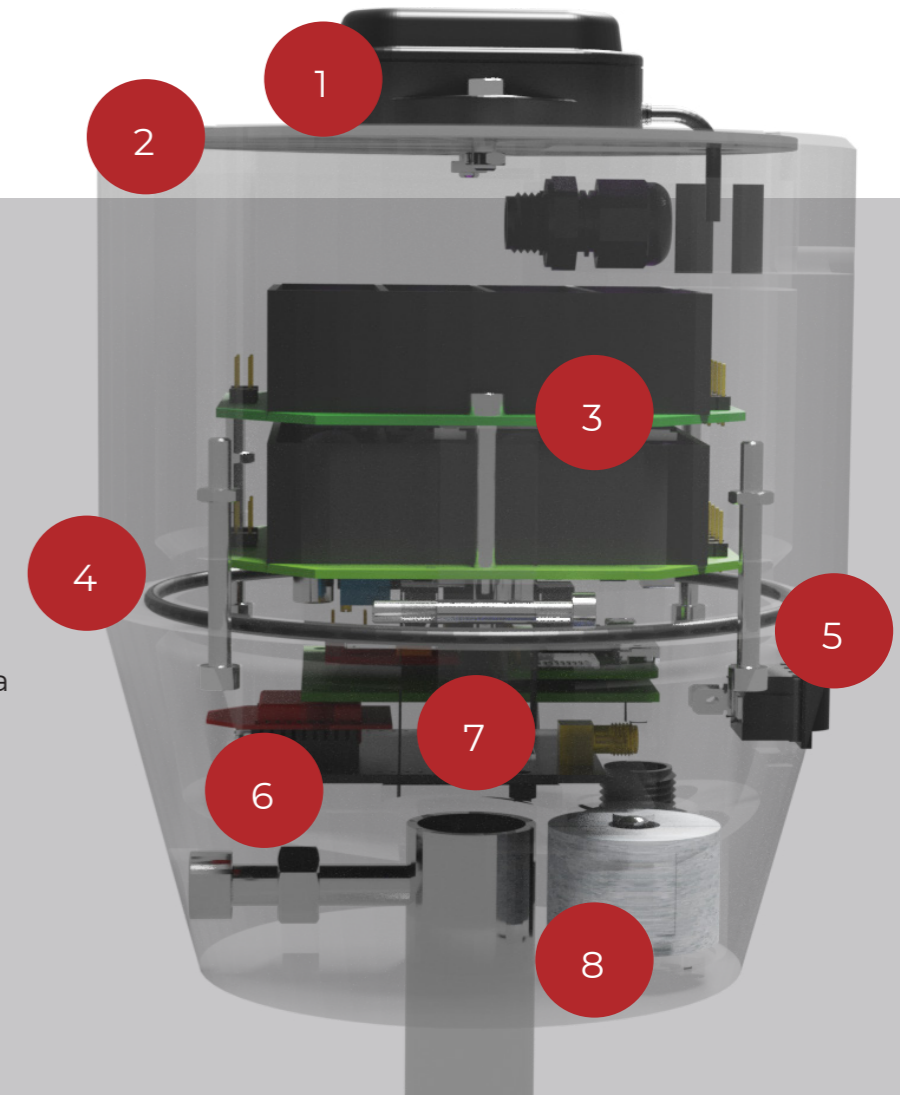
R.2. Look through render of BASE 1
