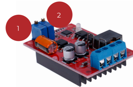
O.6. CN3722 MPPT solar charge controller
