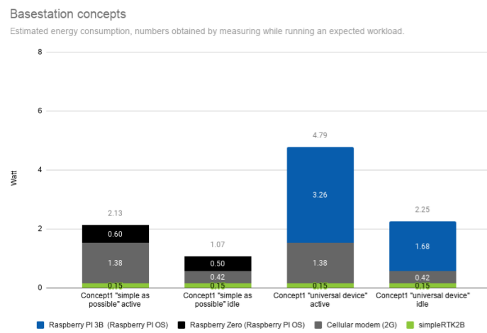
6.6. Power consumption of the concept1 and concept2 base stations in active and idle mode.
