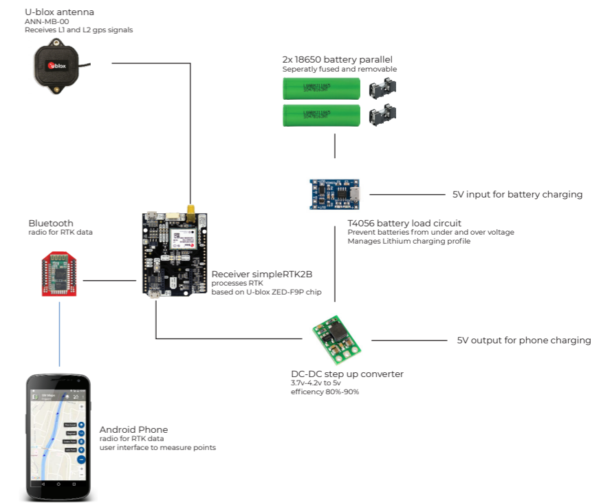
6.8. Hardware structure of final rover design
