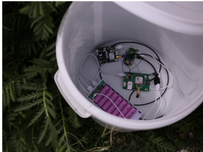
8.4. Base station hardware in a bucket.
