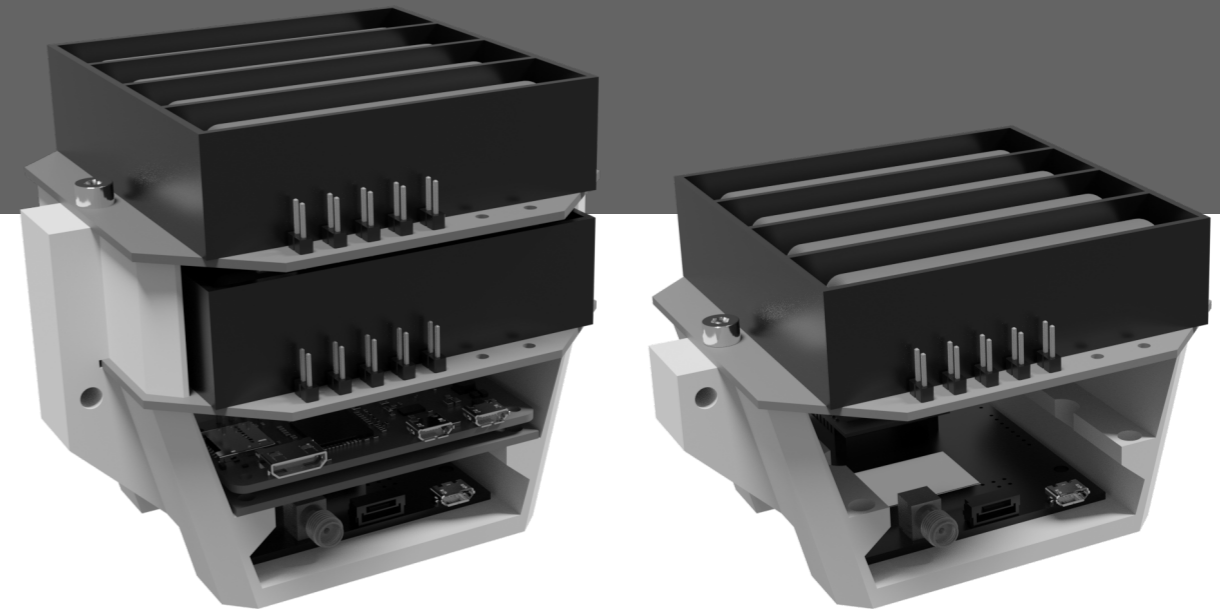
6.34. Electronics assembly of the first intuitive design. Left: BASE1. Right: ROVER1.
