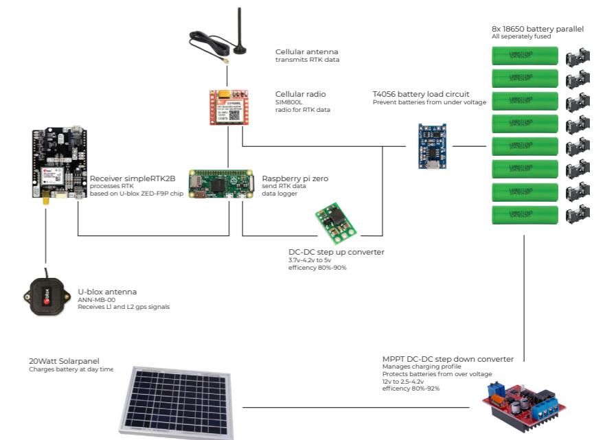
6.9. Hardware structure of final base station design
