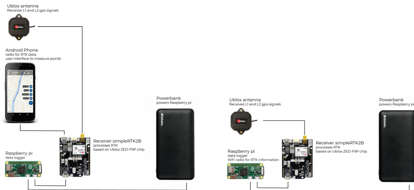
6.1. Initial hardware setup used by previous researchers. Left: Rover, Right: Base Station
