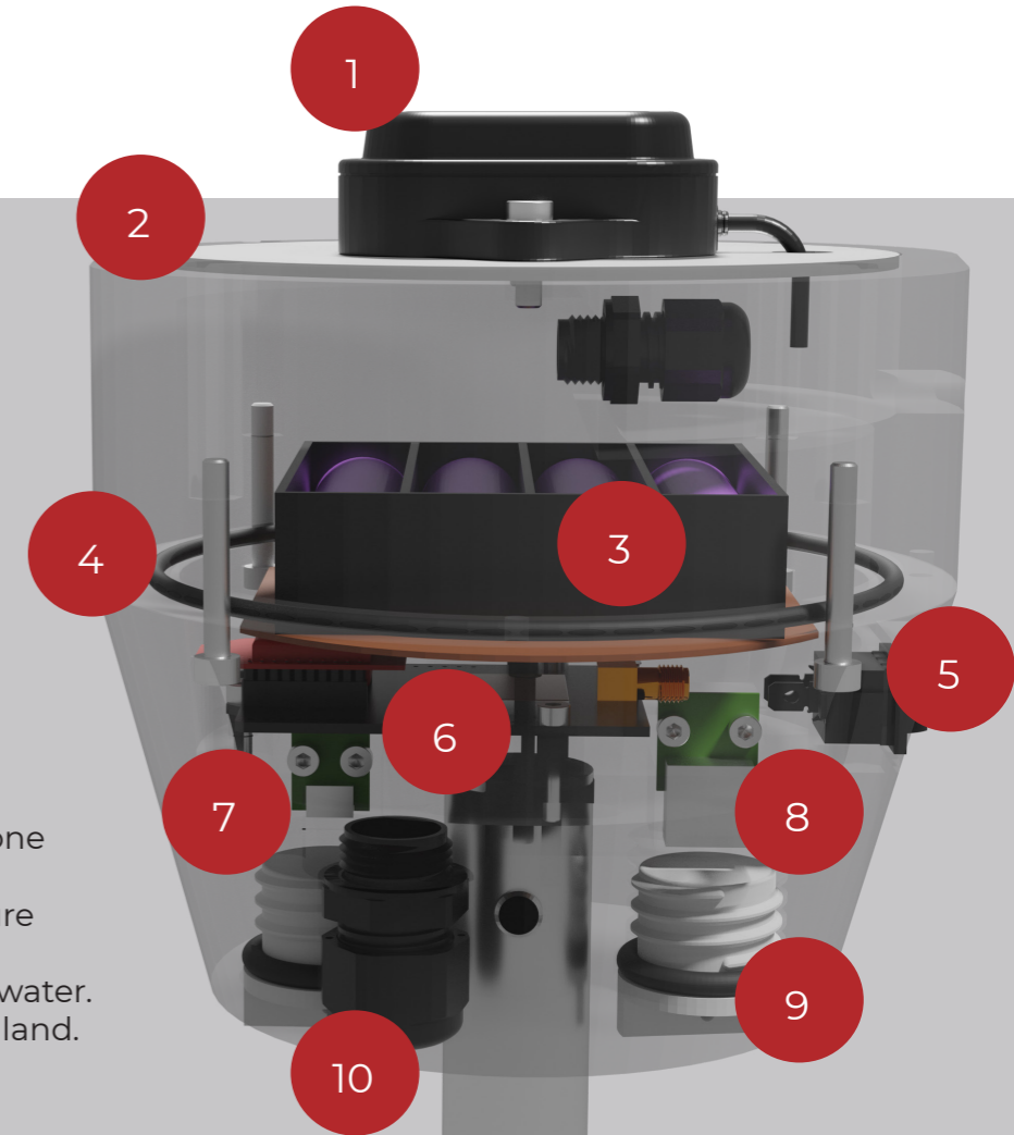
Q.2. Look through render of ROVER1
