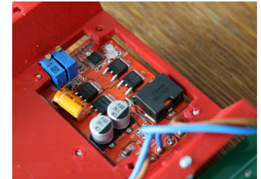
O.7. CN3722 MPPT solar charger mounted in
