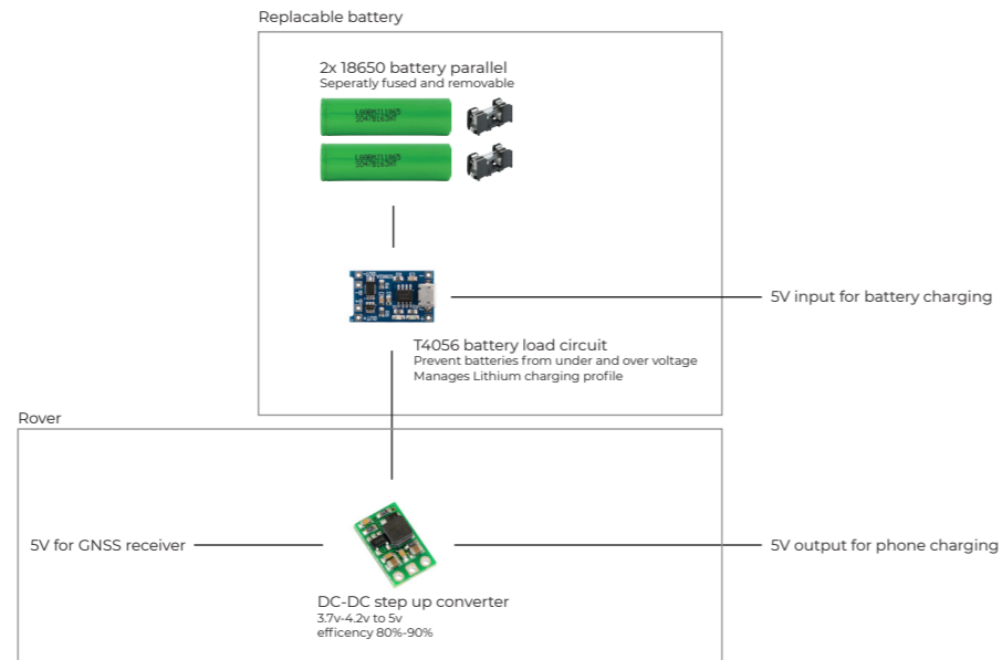
6.35. Final structure of the ROVER2 powersupply →
