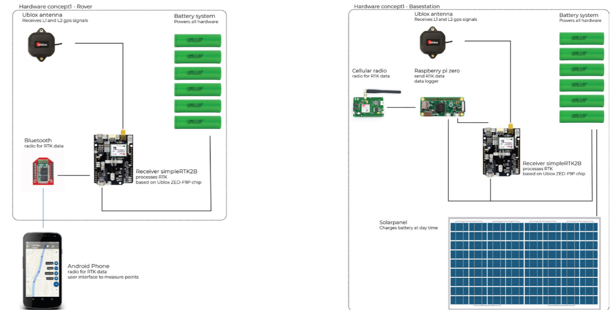
6.2. Hardware concept1. Extending the existing hardware Left: The initial rover hardware extended with a Bluetooth connection to the phone. Right: The initial base hardware extended with a cellular modem and solar-panel.
