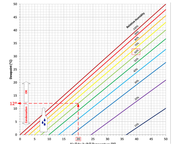
H.1. Chart to determine the dew point based on the Magnus equation (altitude = 0m) (Drexhage, 2016)
