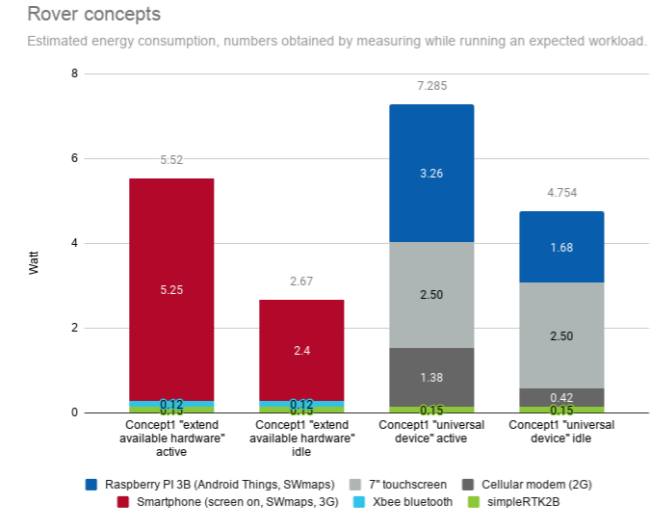
6.7. Power consumption of the concept1 and concept2 rovers in active and idle mode.
