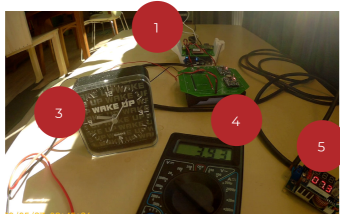
N.1. View from the observing camera: 1. Modem receiver and Raspberry 2. Battery system in the middle 3. Clock for time reference 4. Battery voltage 5. Power meter on the solar dc-dc converter.
