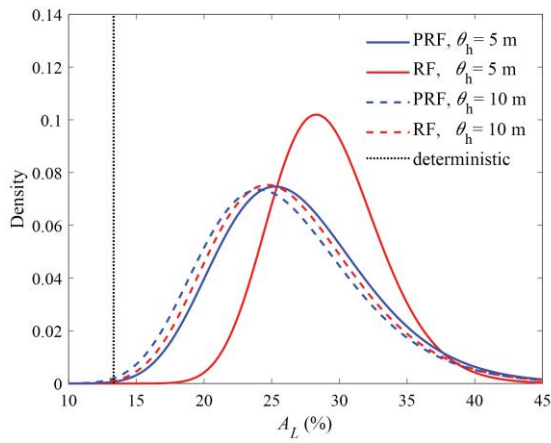
(a) \sigma_e = 0.04
