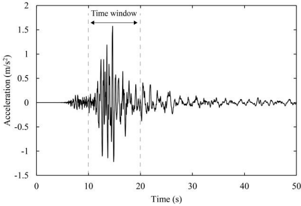
Figure 4. 1999 Chi-Chi earthquake (station CHY074, component 0, PGA = 154.51 cm/s²)
