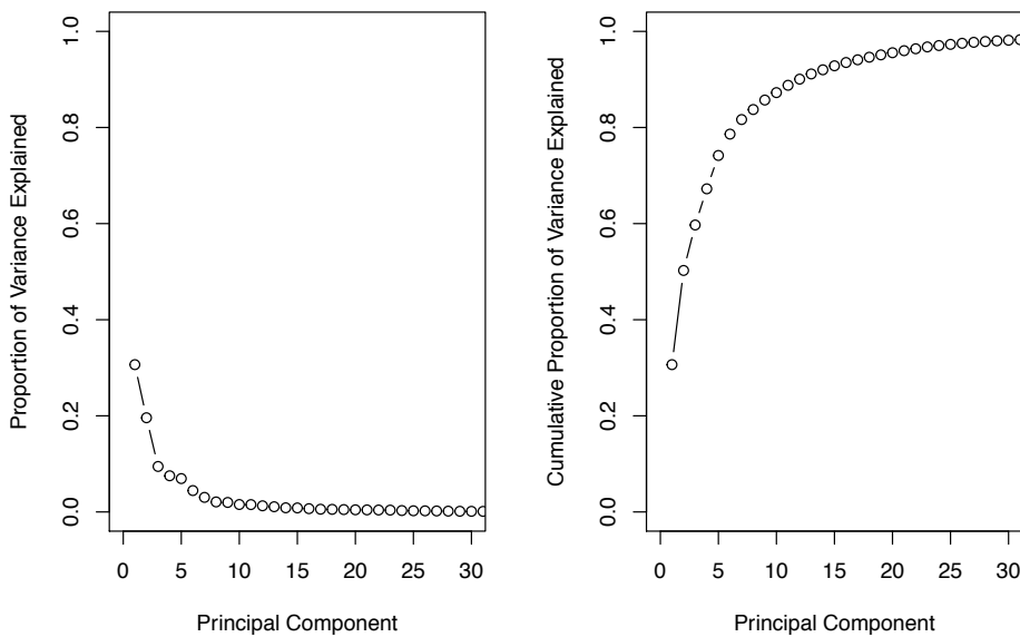
Figure D.1: Plot showing the variance explained by the principal components (both proportion and cumulative proportion) against the number of principal components.
