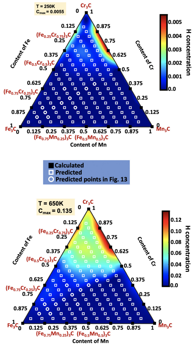
FIG. 14. Heat maps of H concentration in (\text{Fe,Cr,Mn})_3\text{C} carbides at two different temperatures is plotted in the form of a Gibbs triangle. The black-filled squares along the border of the triangle correspond to the H concentration values obtained using ab initio calculations in binary-metal carbides and the white nonfilled squares inside the triangle represent the H concentration values in ternary-metal carbides from the machine learning model. The white nonfilled circles in the triangle correspond to the test set of the model. The projected heat maps of the H concentration are obtained by employing a cubic interpolation scheme on the data points.
