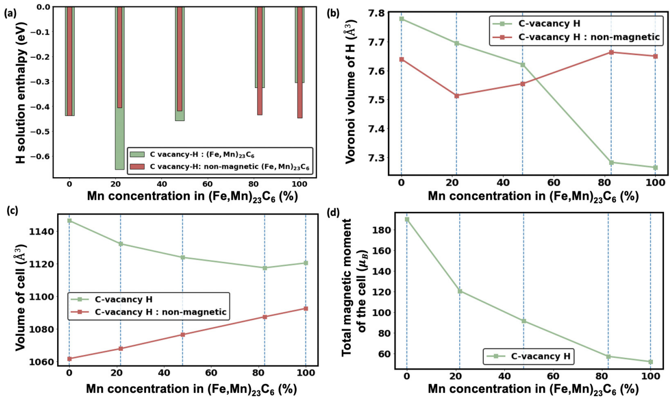
FIG. 8. (a) Calculated solution enthalpies of H at the C vacancy positions in Mn-containing Fe 23 C 6 evaluated both magnetically and nonmagnetically with increasing concentration of Mn. Corresponding changes in (b) the Voronoi volume, (c) the volume of the cell, and (d) the magnetic moment of the cell are examined.
