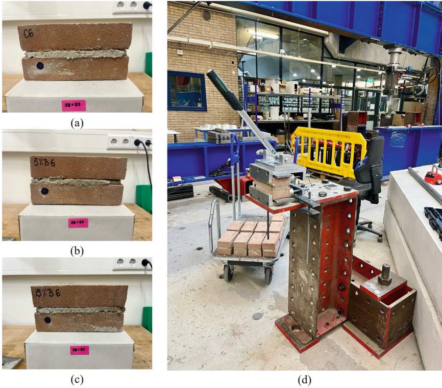
Fig. 1. (a) Reference and bacteria-based masonry couplets at agent concentrations of (b) 5% and (c) 15%; (d) bond wrench test set-up used for testing.
