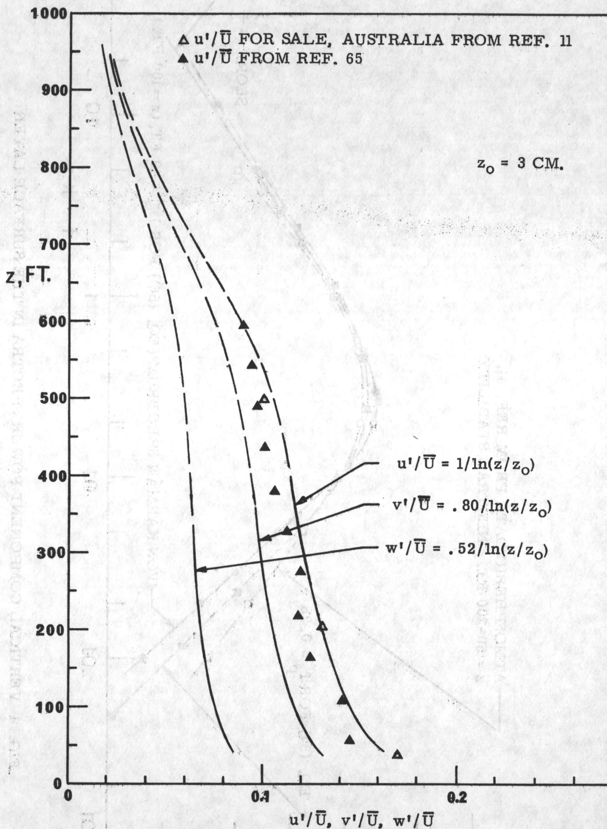
FIG. 3 TURBULENCE INTENSITY VARIATION WITH HEIGHT IN NEUTRAL STABILITY OVER FLAT TERRAIN
