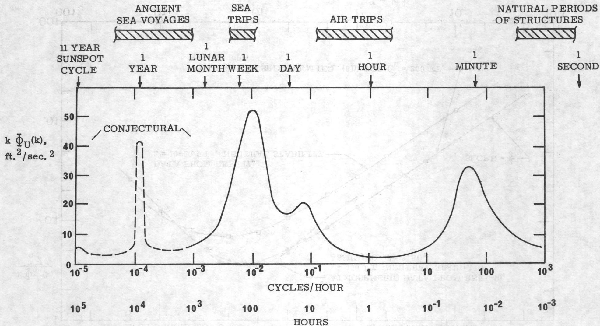
FIG. 5 SPECTRUM OF WIND SPEED AT BROOKHAVEN, U. S. A. (FROM REF. 30)
