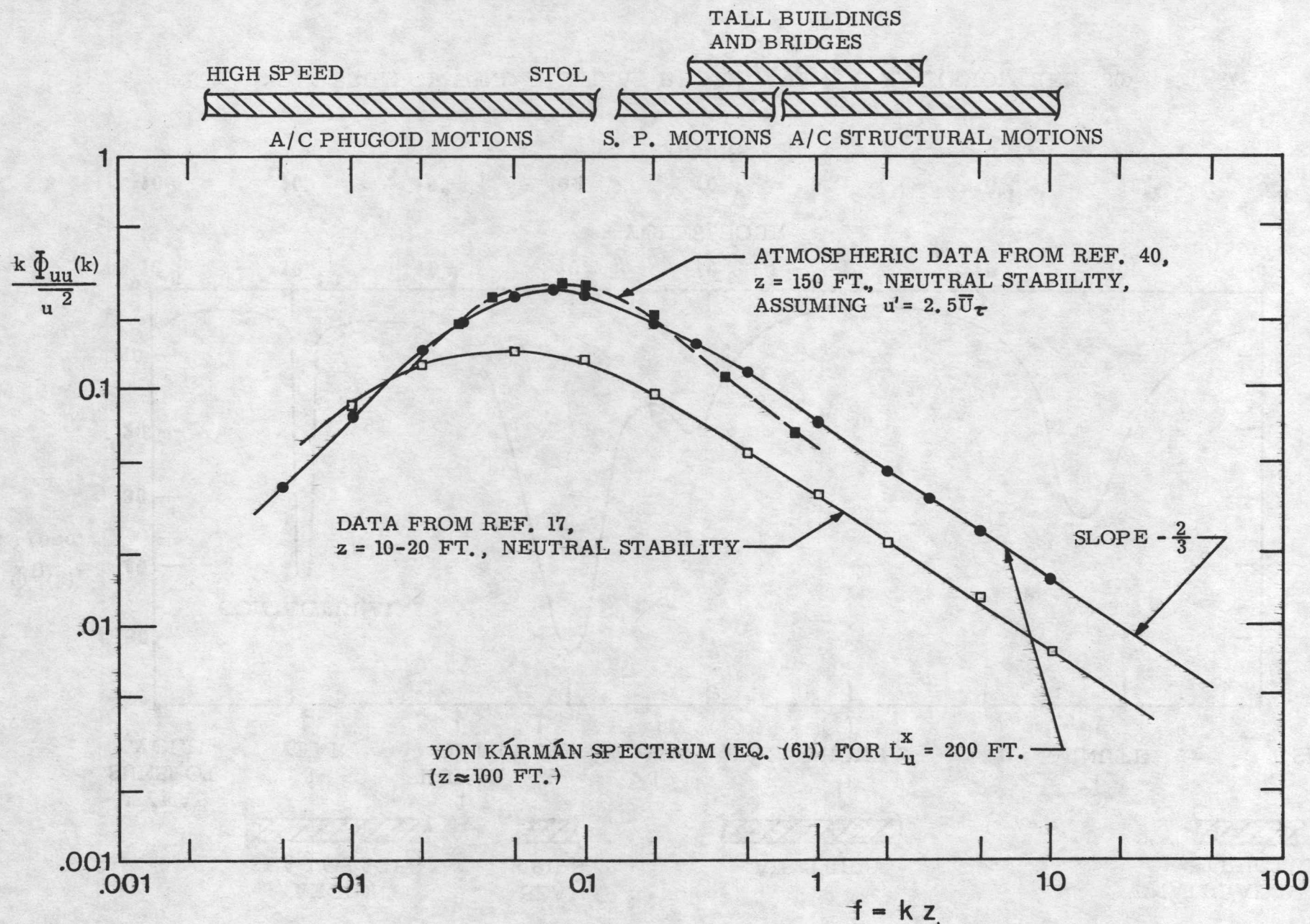
FIG. 6 LONGITUDINAL COMPONENT POWER SPECTRA IN THE SURFACE LAYER
