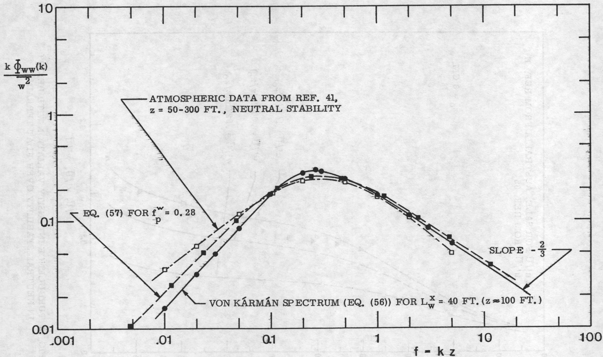
FIG. 4 VERTICAL COMPONENT POWER SPECTRA IN THE SURFACE LAYER
