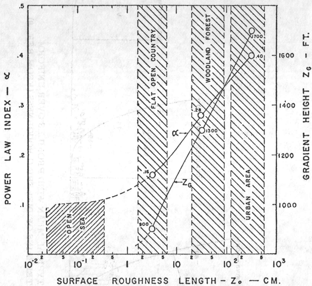
FIG. 1 PARAMETERS OF THE POWER LAW FOR MEAN WIND VELOCITY (FROM REF. 9)
