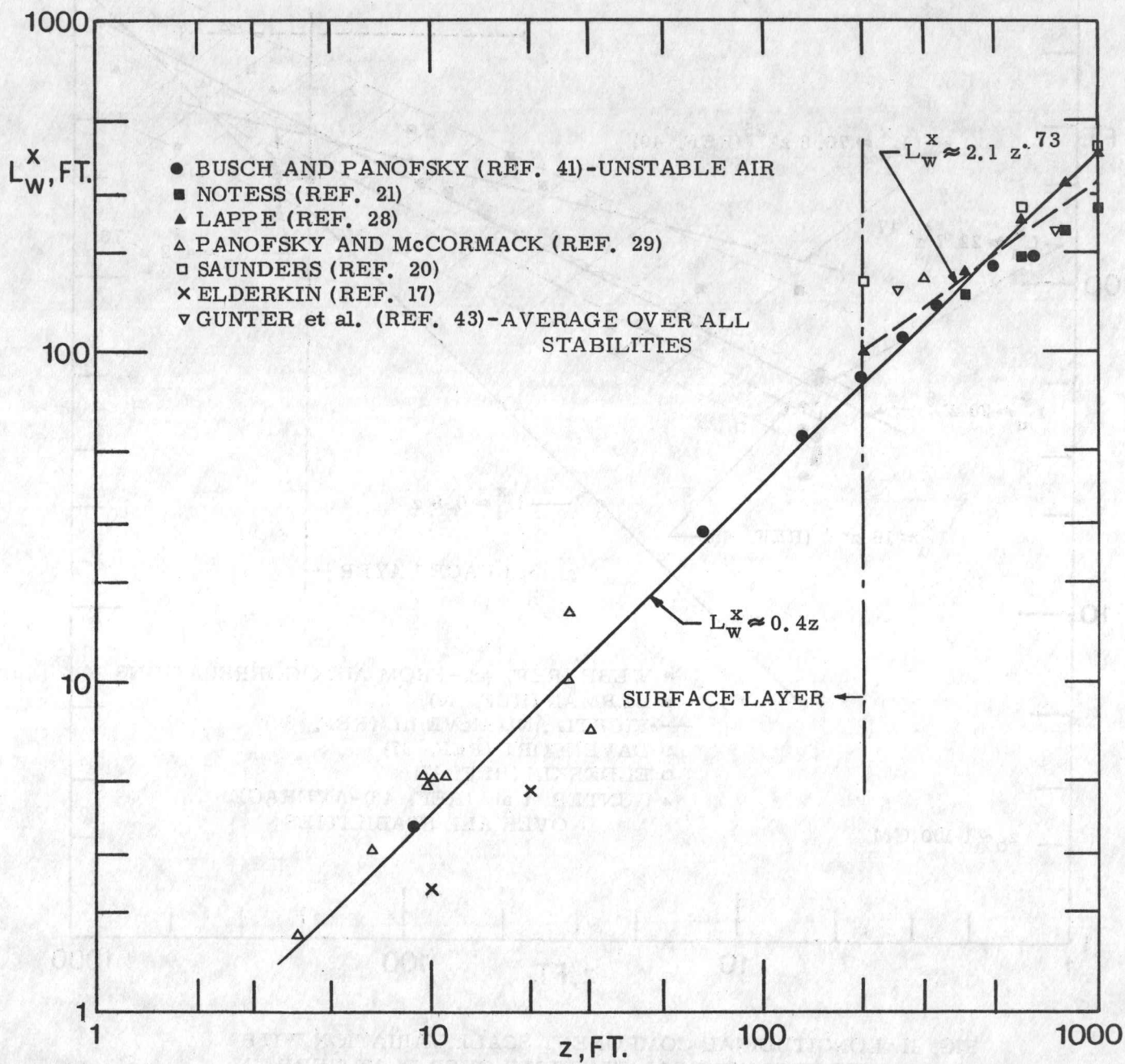
FIG. 10 VERTICAL COMPONENT SCALE VARIATION WITH HEIGHT IN NEUTRAL STABILITY OVER FLAT TERRAIN
