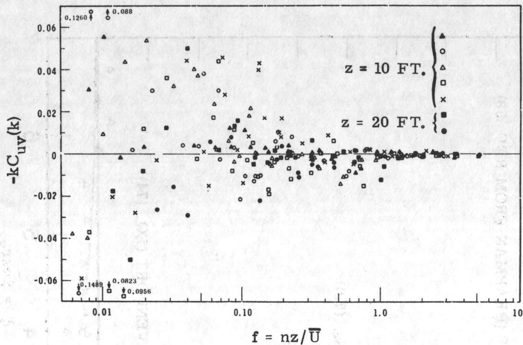
FIG. 7 COSPECTRA BETWEEN LONGITUDINAL AND LATERAL VELOCITY-NEUTRAL STABILITY
