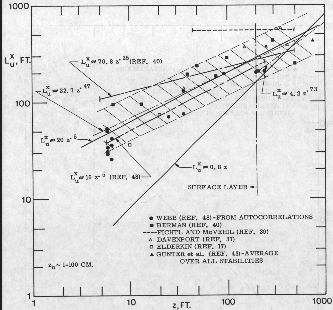
FIG. 11 LONGITUDINAL COMPONENT SCALE VARIATION WITH HEIGHT IN NEUTRAL STABILITY OVER FLAT TERRAIN
