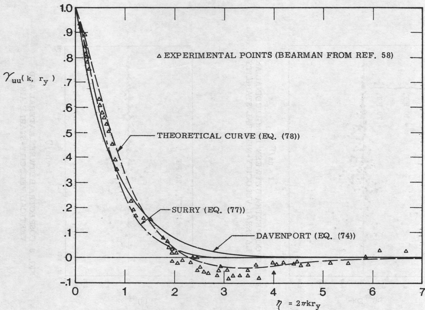
FIG. 9 CROSS-CORRELATION SPECTRA FOR GRID-GENERATED TURBULENCE
