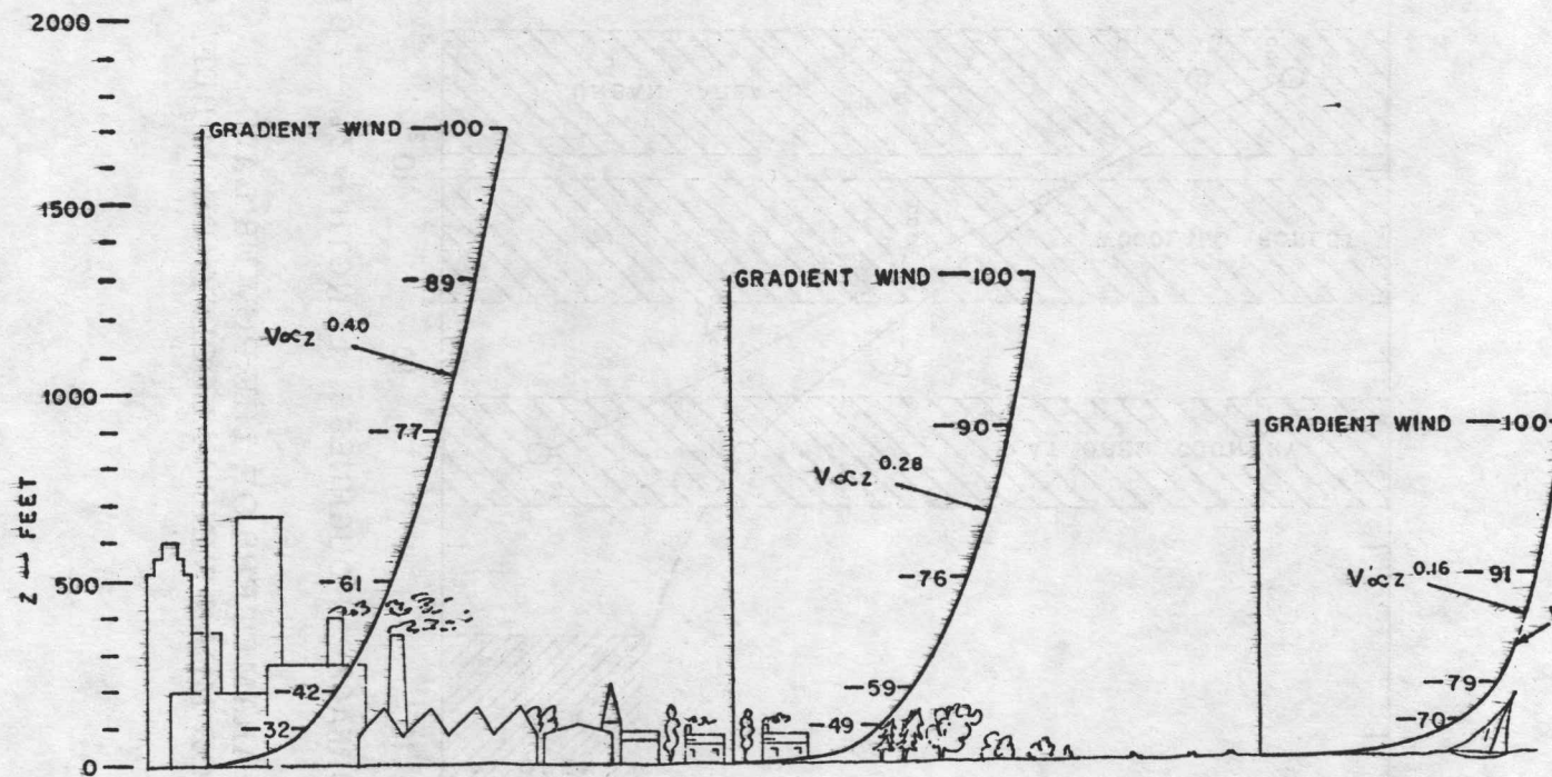
FIG. 2 TYPICAL MEAN WIND PROFILES OVER UNIFORM TERRAINS OF DIFFERING ROUGHNESS (FROM REF. 9)
