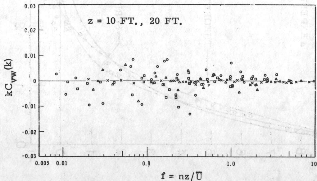
FIG. 8 COSPECTRA BETWEEN LATERAL AND VERTICAL VELOCITY-STABLE AIR
