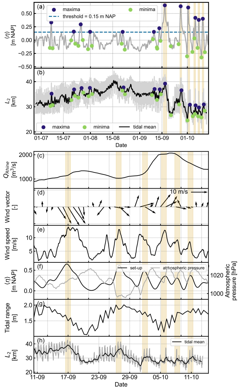
Figure 6. Overview of the selected coastal set-up events, including (a) coastal set-up at Hoek van Holland \langle \eta \rangle (meters above NAP) and (b) salt intrusion length L_2 (km). The yellow highlighted events are zoomed in upon with additional parameters. (c) Rhine River discharge Q_{Rhine} ( m^3/s ). (d) The daily mean wind vector. (e) \langle \eta \rangle (meters NAP) and atmospheric pressure (hPa) at Hoek van Holland. (f) The tidal range (m) at Hoek van Holland. (g) L_2 (km). The yellow areas highlight 48 hr around the maximum set-up.
