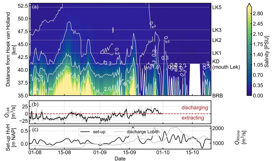
Figure 8. (a) Salinity contours (PSU) in the New Meuse and Lek, between salinity stations BRB and LK5. The salinity values are interpolated between the stations, whose locations are indicated by white dotted lines. (b) Discharge through the Lek Q_{Lek} ( \text{m}^3/\text{s} ), where positive values represent a net freshwater discharge on the Lek and negative values net extractions from the Lek. (c) Set-up \langle \eta \rangle (m NAP) at Hoek van Holland and Rhine River discharge Q_{Rhine} ( \text{m}^3/\text{s} ).
