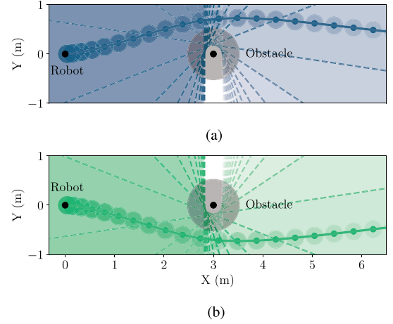
Fig. 5. Two distinct locally planned trajectories for a robot (black dot) evading an obstacle (black region and dot) that is static ( \mathcal{O}_k = \mathcal{O}_0, k = 1, \dots, N ). For both planners, we depict the topology constraints for each time step in their respective colors showing the constraint boundaries (broken lines) and their feasible region (colored regions with increasing transparency over time). (a) Local planner 1 plans to evade the obstacle left. (b) Local planner 2 plans to evade the obstacle right.
