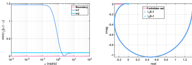
Figure 3. Alternative visualisations of the stability condition (13) in Theorem 2, for the system in Example 3. Left: the two blue lines are \min_{\rho \leq -(2\mathfrak{D})-1} |\lambda_i(j\omega) - \rho| for i = 1, 2 , with \mathfrak{D} = 5 . The condition for nominal topology-independent stability is that they are strictly above zero, which is violated. Right: for nominal stability, the curves \lambda_1(j\omega) and \lambda_2(j\omega) should never intersect the forbidden set \mathcal{S} = \{z \in \mathbb{R} : z \leq -0.1\} ; the condition is violated.
