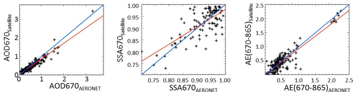
Figure 10. Comparison of GRASP/PARASOL retrieved parameters AOD, AE and SSA at 670 nm vs. AERONET station measurements over sites Mongu, Banizoumbou, IER_Cinzana, Agoufou, Ilorin, DMN_Maine_Soraa in Africa for 2008. The red lines show the linear regression fit.
