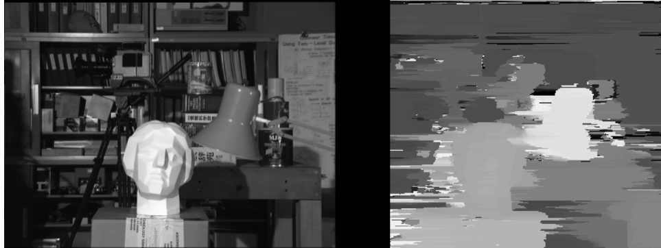
Figure 2. Tsukuba image from the Middlebury stereo benchmark and the resulting disparity map from our simplified implementation of [29].
