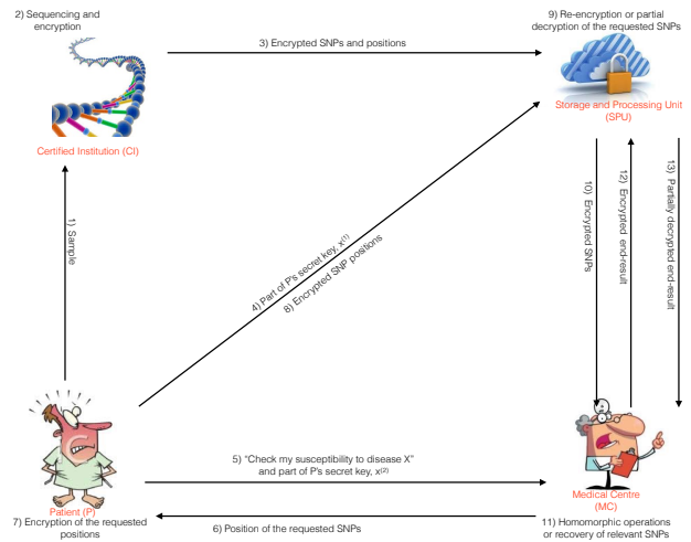
Figure 1: Protocol proposed by Ayday et al.[4]
