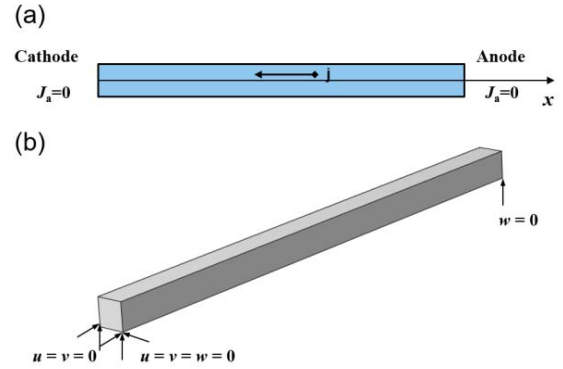
Figure 4. (a) Schematic for a stress-free Al line. (b) Applied constraints for conductor in FEA simulation.
