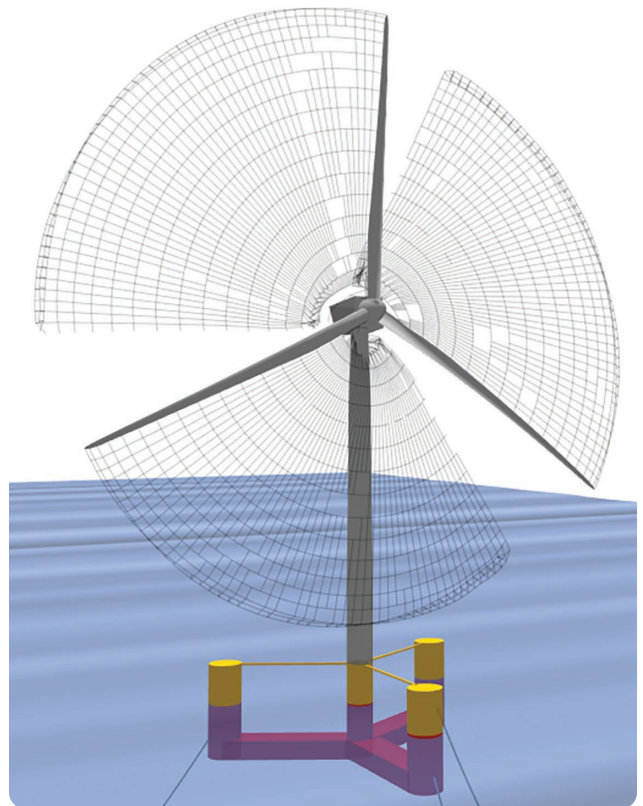
FIGURE 7 A close-up of the IEA 15-MW turbine on the VoltturnUS-S floater in QBlade. The image is taken at the start of the simulation at which only the near wake is visible, represented by the black lines, which are vortex elements released in the wake.
