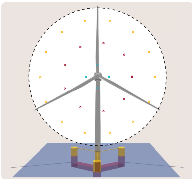
FIGURE 10 The front view of the IEA 15-MW turbine mounted on the VoltornUS-S platform with the points at which the wind speed is measured. The rotor-swept area is indicated by the dashed circle.
