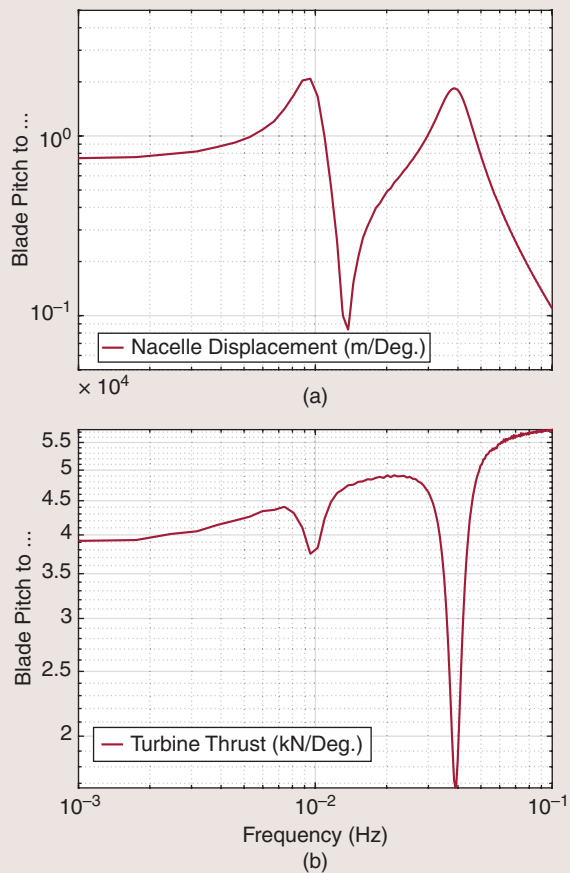
FIGURE S10 (a) and (b) The resulting spectra of the identification experiment for the Pulse wake mixing technique on the OC3 floating turbine. This turbine has two eigenfrequencies and one antiresonance in its nacelle displacement. At the eigenfrequencies, a reduction in the variation of thrust can be seen.
