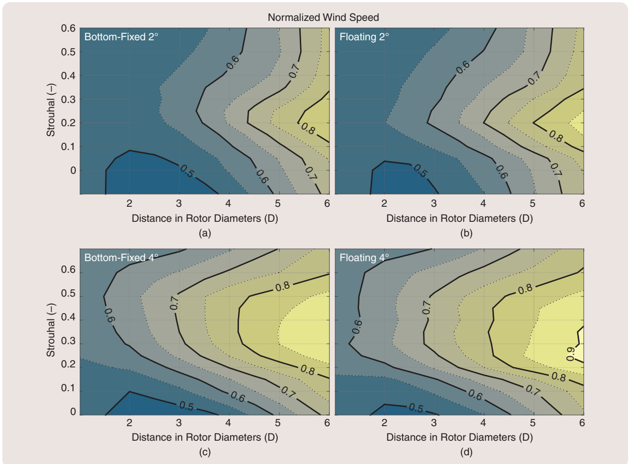
FIGURE 18 The absolute wind farm velocity normalized with V_\infty = 9 m/s. Between S_t = 0.3 and S_t = 0.35 , the gain in wind speed is the highest for both types of turbines. Increasing the blade pitch amplitude increases the frequency range at which higher wind speeds can be achieved. (a) Bottom-fixed 2°. (b) Floating 2°. (c) Bottom-fixed 4°. (d) Floating 4°. (Source: Color map courtesy of [80].)
