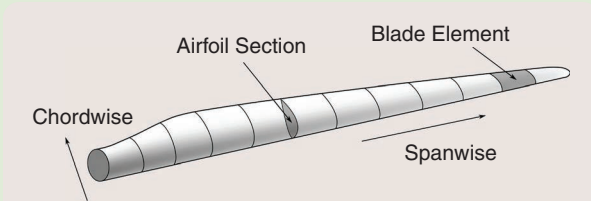
FIGURE S2 2D airfoil sections and the discretization of a rotor blade into 2D elements.
