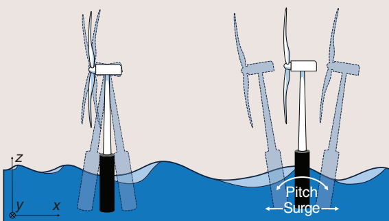
FIGURE S9 An example of how a similar platform pitch and surge motion can result in a different nacelle displacement.
