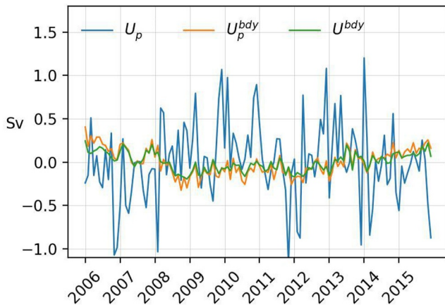
Figure 11. Volumetric flow across the 200 m isobath due to the along-isobath pressure gradient in the reference experiment, U_p , and bdy experiment, U_p^{bdy} . Also shown is the total volumetric flow across the 200 m isobath in the bdy experiment, U^{bdy} .
