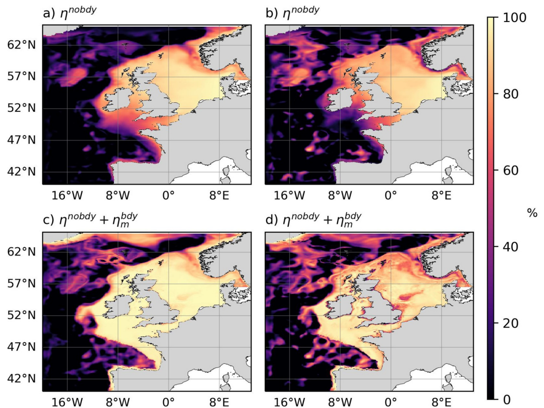
Figure 6. Percentage of variance explained in reference model dynamic sea level (DSL) by: (a) the DSL from the nobdy experiment, \eta^{nobody} , and (c) the sum of the DSL from the nobdy experiment, \eta^{nobody} , and the manometric sea level from the bdy experiment, \eta_m^{bdy} , that is, \eta^{nobody} + \eta_m^{bdy} . Panels (b) and (d) show the same as (a) and (c), respectively, but with 12-month rolling means applied.
