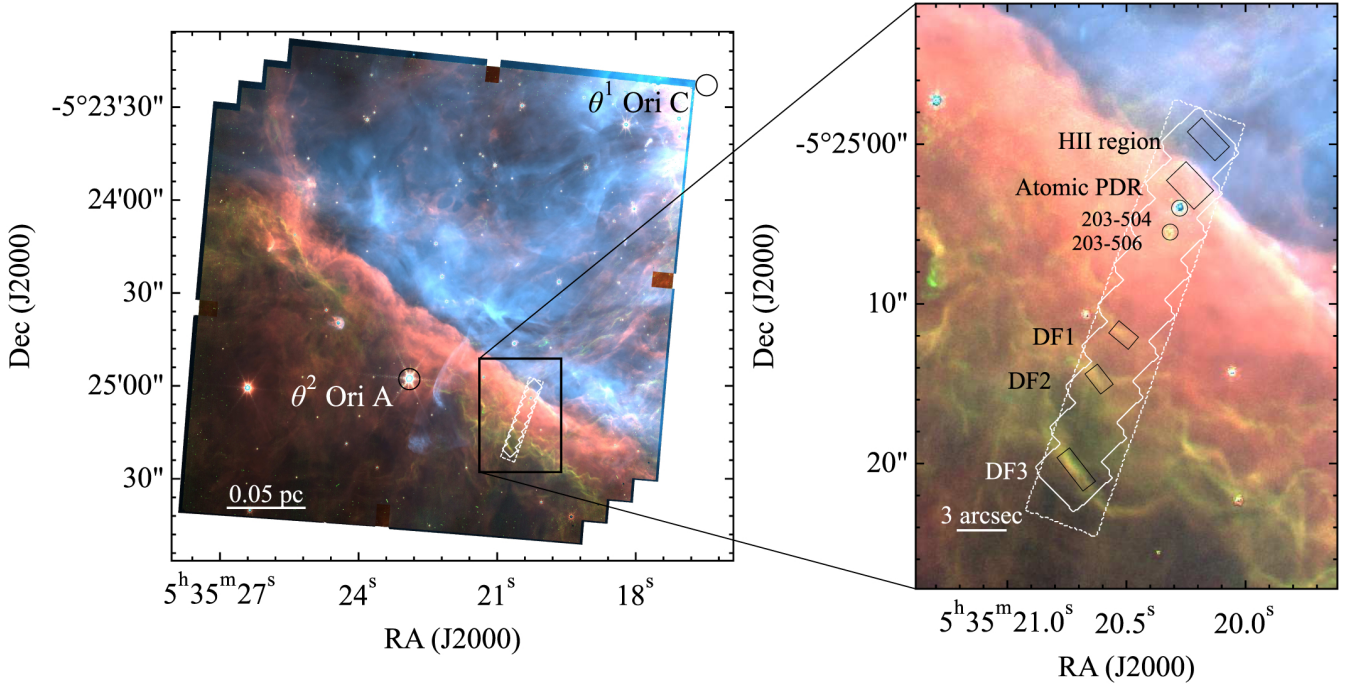
Fig. 1. PDRs4All MIRI MRS and NIRSpec footprints (dashed and solid white boundaries, respectively), and spectral extraction apertures (black boxes in the right panel) on top of a composite NIRC2 image of the Orion Bar (data from Habart et al. 2023). DF 1, DF 2, and DF 3 are \text{H}_2 dissociation fronts as designated in Habart et al. (2023). Red, green, and blue are encoded as F335M (AIB), F470N–F480M ( \text{H}_2 emission), and F187N (Paschen \alpha ), respectively.
