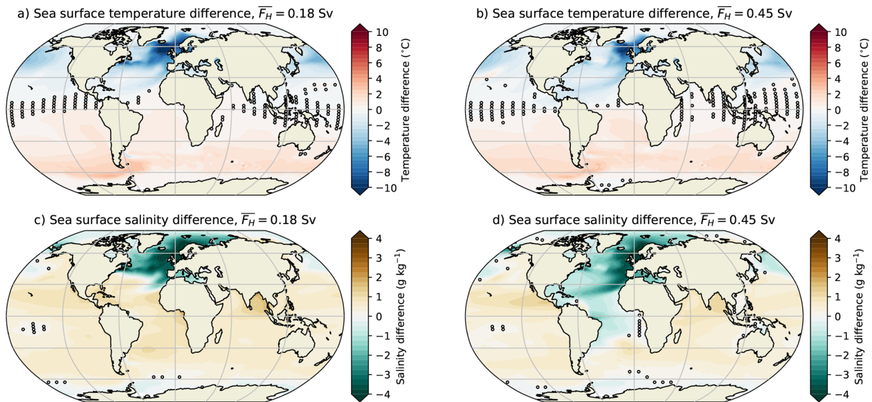
Figure A3. (a, b) Sea surface temperature differences between the statistical equilibria for \overline{F_H} = 0.18 Sv and \overline{F_H} = 0.45 Sv, displayed as the “AMOC off” state minus the “AMOC on” state. (c, d) Sea surface salinity differences between the statistical equilibria for \overline{F_H} = 0.18 Sv and \overline{F_H} = 0.45 Sv, displayed as the “AMOC off” state minus the “AMOC on” state. The markers indicate non-significant ( p \geq 0.05 ) differences.
