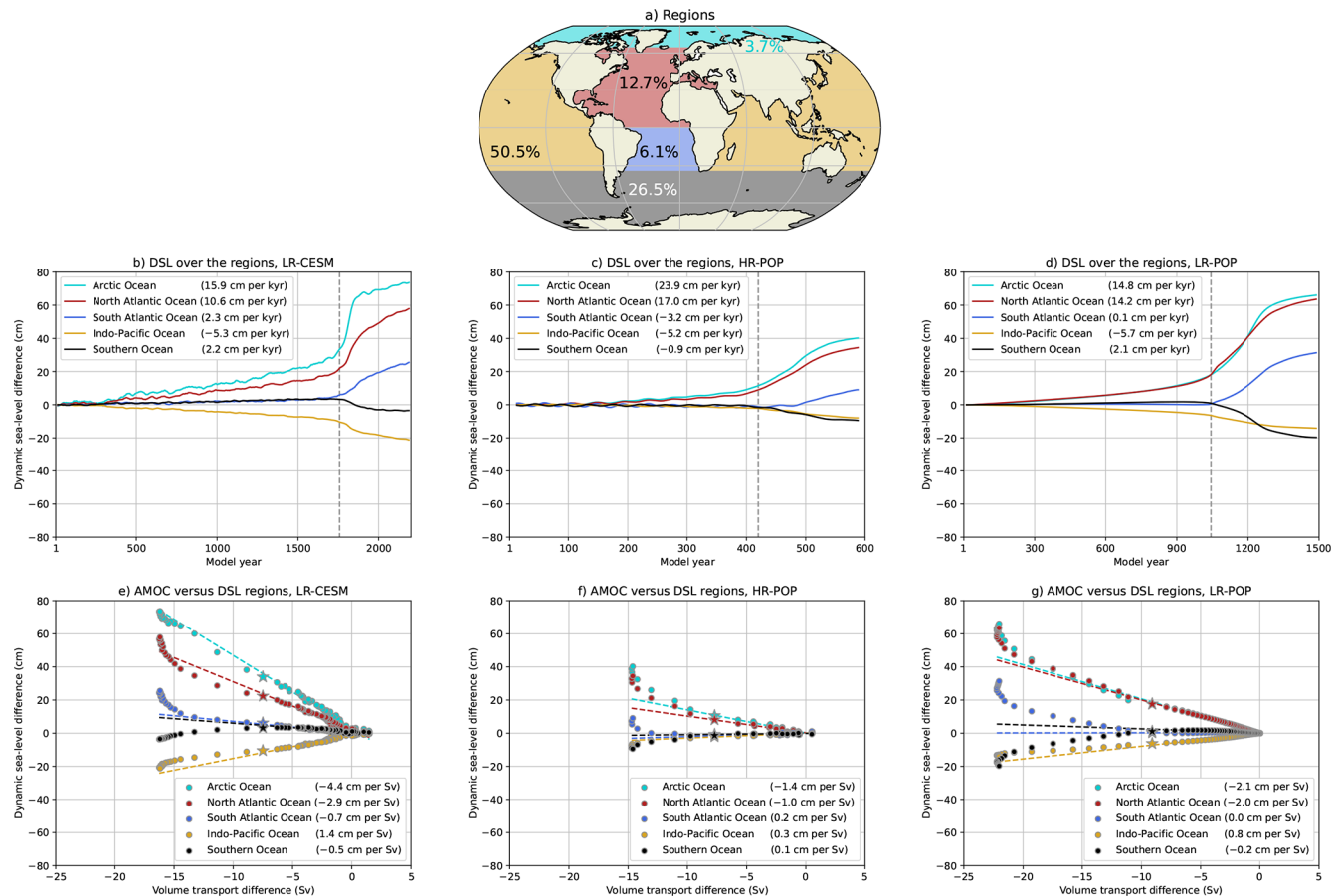
Figure 2. (a) Definition of the five different regions. The percentages indicate the fraction of the total ocean surface, the remaining 0.5 % is attributed to (semi-)enclosed seas and lakes. (b–d) Spatially-averaged DSL over five different regions for the LR-CESM, HR-POP and LR-POP. The DSL time series are displayed as their differences to the first 50 years and are then smoothed through a 25-year running mean to reduce the variability. The vertical gray line marks the onset of the AMOC collapse. The DSL trends are determined from model year 1 up to the AMOC tipping event and given in the legend ( \nu ). (e–g) Relation between AMOC strength and DSL by region for the LR-CESM, HR-POP and LR-POP. The AMOC strength and DSL by region are displayed as their differences to the first 50 years and are shown for 25-year windows, the star marker indicates the window of the onset of the AMOC collapse. A linear fit is determined through these 25-year windows, starting from the first window up to the window with the star marker, and are given in the legend ( \phi ).
