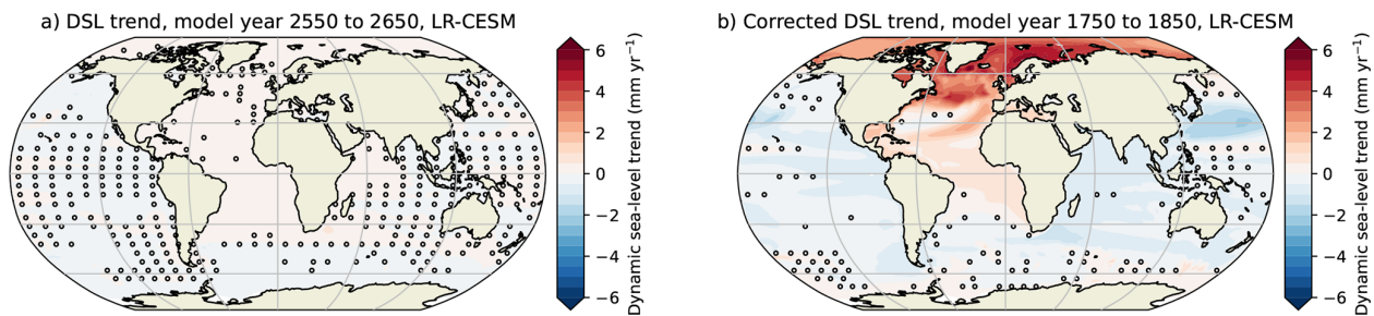
Figure 7. (a) DSL trends over model years 2550–2650 for the LR-CESM. Note that the sign of the DSL trends is reversed. (b) The hosing-corrected DSL trends for model years 1750–1850 for the LR-CESM. Markers indicate non-significant ( p \geq 0.05 ) DSL trends.
