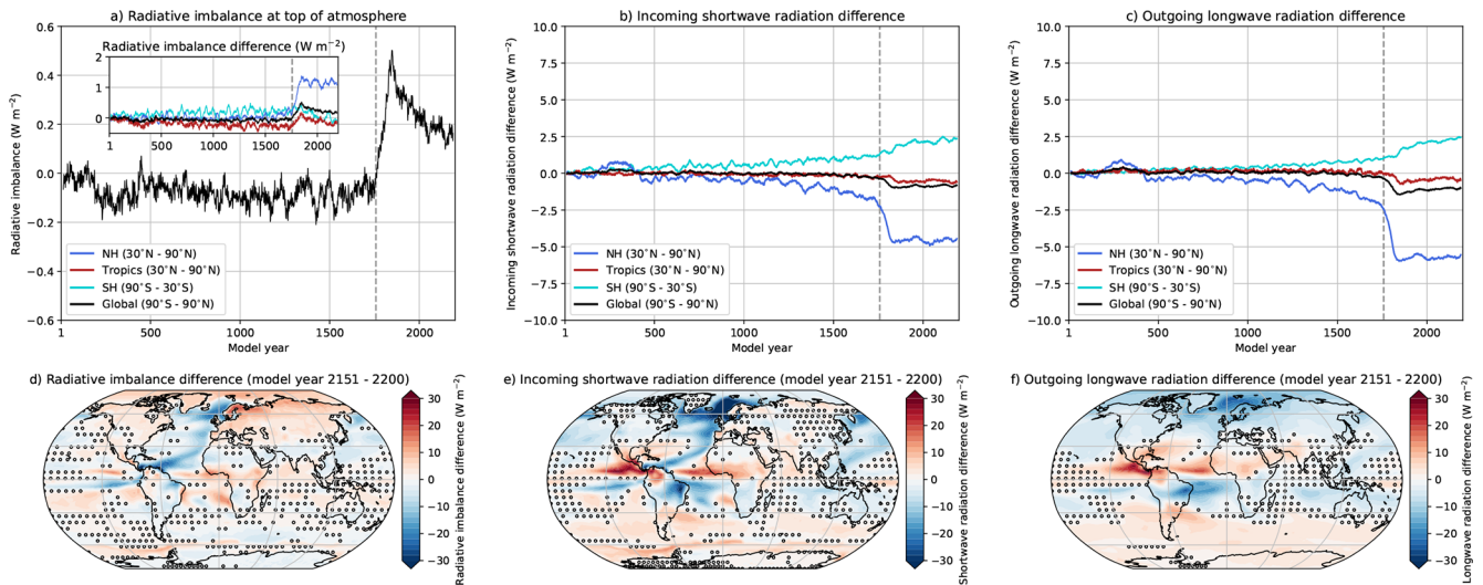
Figure 10. (a–c) The globally-averaged radiative imbalance at the top of atmosphere (a) for the LR-CESM. The inset shows the radiative imbalance difference compared to first 50 model years, which is also split for different latitude bands. The radiative imbalance is decomposed into an incoming shortwave radiation ( SW^{\text{in}} , panel (b)) contribution and outgoing longwave radiation ( LW^{\text{out}} , panel (c)) contribution. The SW^{\text{in}} and LW^{\text{out}} time series are displayed as differences (compared to the first 50 model years) and for different latitude bands. All time series are smoothed through a 25-running mean to reduce the variability. The dashed gray line indicates the onset of the AMOC collapse. (d–f) The radiative imbalance at top of atmosphere, SW^{\text{in}} and LW^{\text{out}} differences for model years 2151–2200 (compared to first 50 model years). The markers indicate non-significant ( p \geq 0.05 ) differences.
