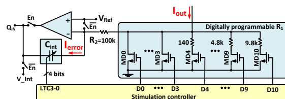
Fig. 3: Schematic diagram of the sensing circuits.
