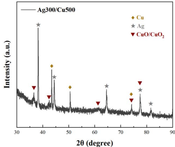
Figure 8. The result of XRD of sample Ag300/Cu500 after soaking in NaCl solution for 28 days
