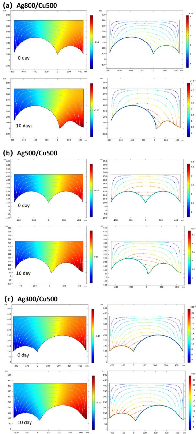
Figure 4. The simulation results of the electrolyte potential (left column / V) and current density vector distribution (right column / \text{A}\cdot\text{m}^{-2} ) of the three groups of particle size combinations at initial and after 10 days of corrosion: (a) R_{\text{silver},1}=400\text{ nm} ; (b) R_{\text{silver},2}=250\text{ nm} ; (c) R_{\text{silver},3}=150\text{ nm} .
