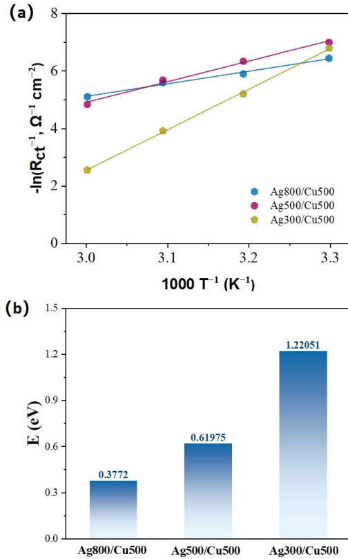
Figure 10. (a) Arrhenius plots of R_{ct} values and (b) the activation energy for 3 kinds of Cu-Ag composite sintered samples.
