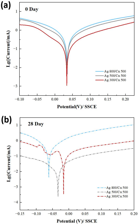
Figure 9. The polarization curves of the sintered samples in NaCl solution before and after corrosion for 28 days
