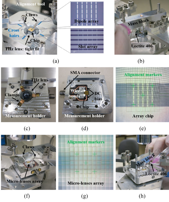
Fig. 5. Assembly procedure. (a) THz lens and array chip mounted into the auxiliary alignment tool. (b) Mass block placed on top of the chip during the glueing to prevent the creation of an air gap between the THz lens and the array chip. (c) Front view of the experiment holder with the THz lens and array chip assembly mounted in it. This assembly is kept in place with three clamps. (d) Back view of the experiment holder with the THz lens and array chip assembly mounted in it. The dc bias lines are connected to the chip with wire bonds. (e) Microscope on-screen markers for the center and the four corners gap elements of the array. (f) Alignment of the microlenses array with the antenna array. (g) Microscope on-screen markers to align the microlenses array with the antenna array. (h) Mass block placed on top of the microlenses array during the glueing to assure that no glue goes under the microlenses array.
