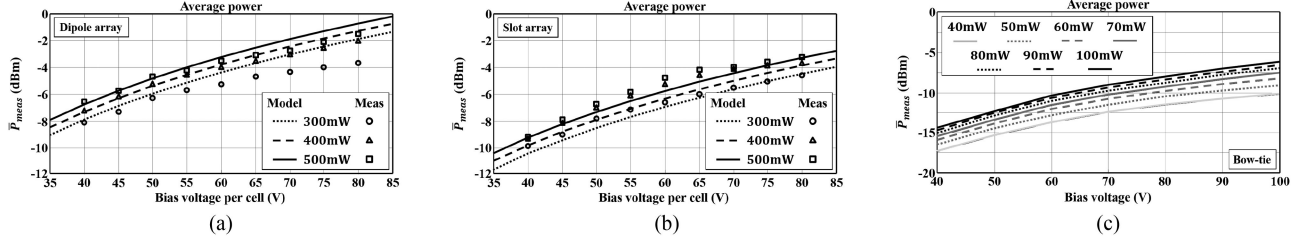
Fig. 11. Measured average power and estimated average detected power \bar{P}_{\text{meas}} of the PCCA prototypes versus the bias voltage applied on the gaps. (a) Dipole array. (b) Slot array. (c) Measured average power of the bow-tie antenna versus bias voltage for different laser power excitations.
