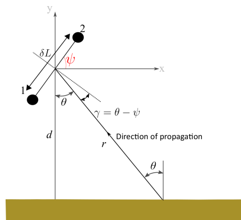
Figure 1. Geometry of interferometry. \theta is the direction of the incoming signal relative to the surface normal.
