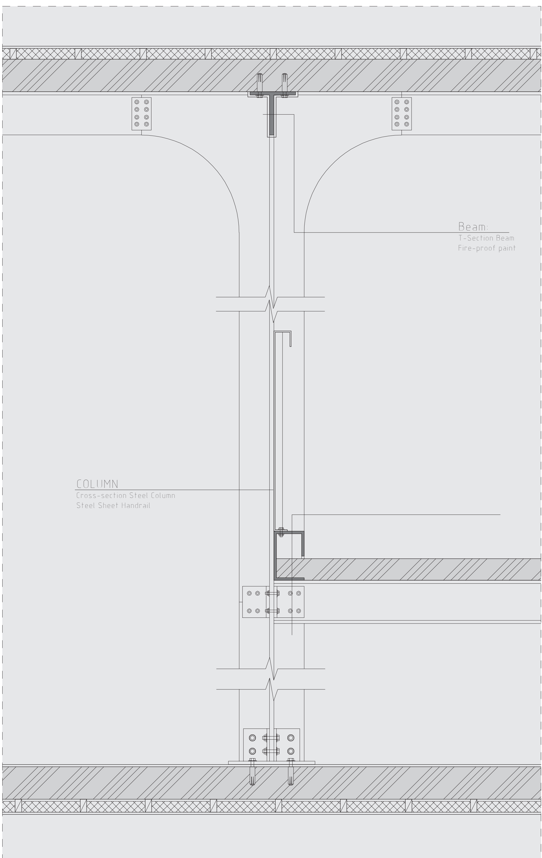
DETAIL-CORNER 4 110
