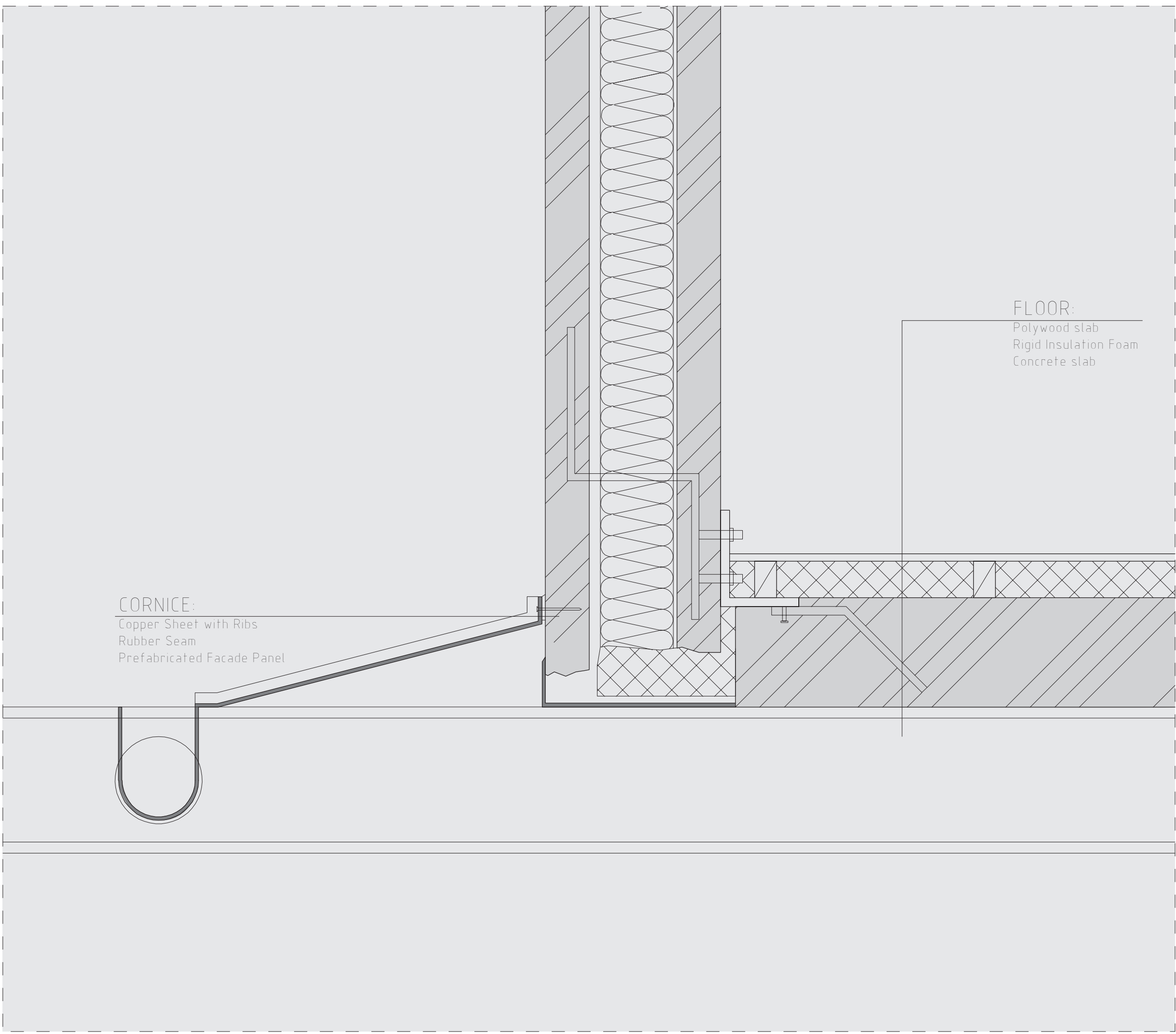
DETAIL-CORNER 3 15
