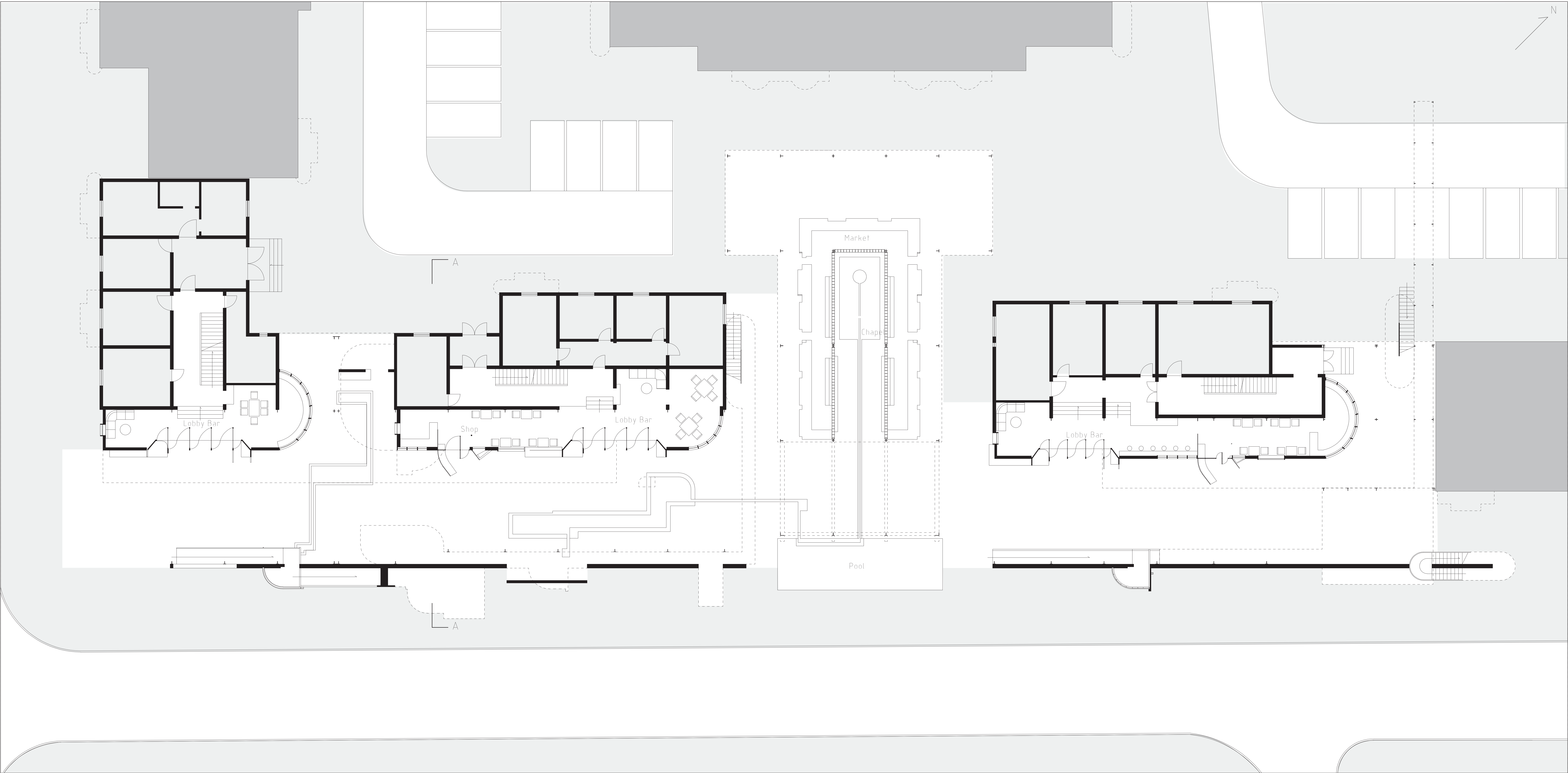
GROUND FLOOR PLAN 1:100
