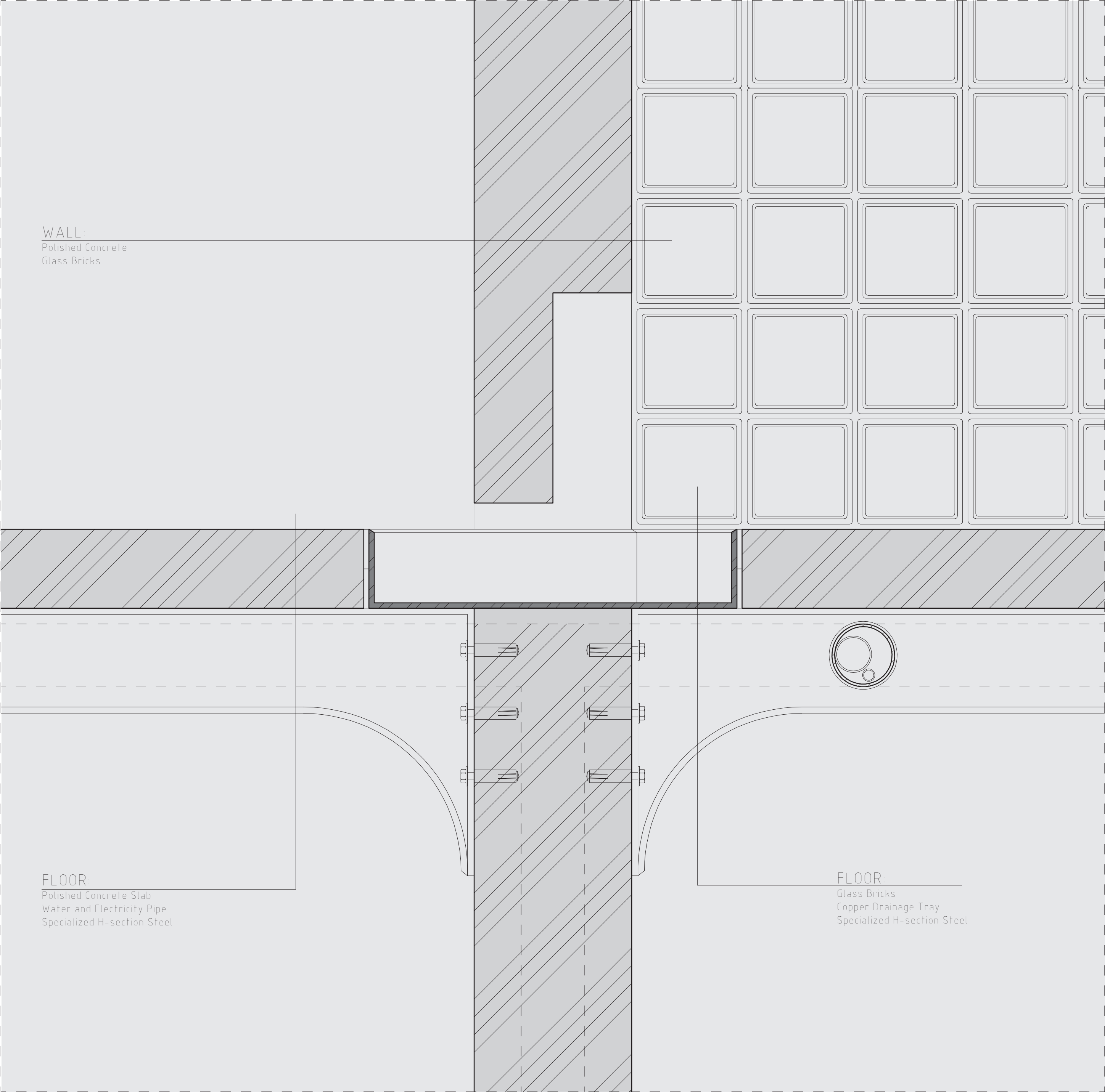
DETAIL-CORNER 1 1:5
