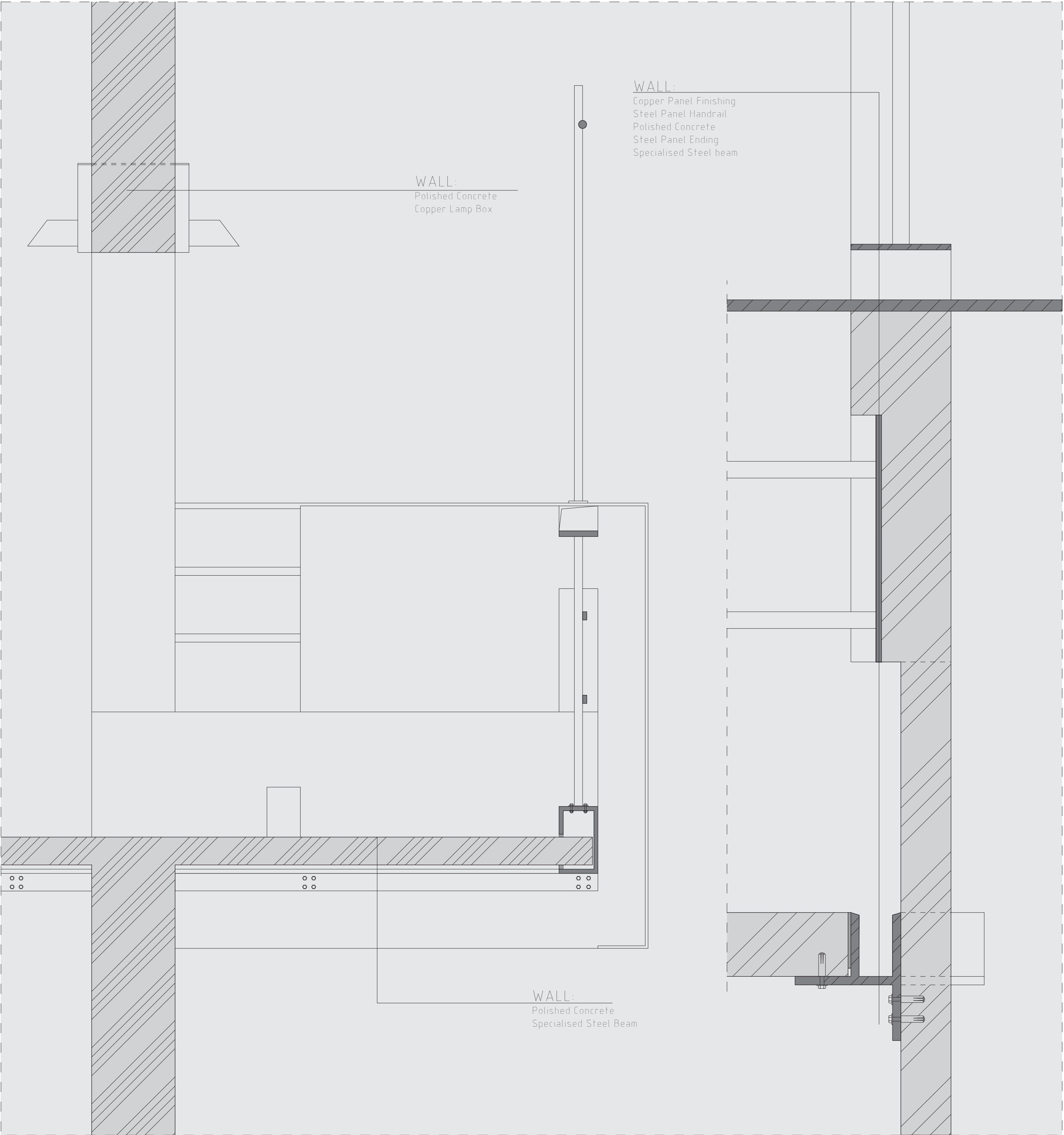
SECTION-CORNER 2 1:10
