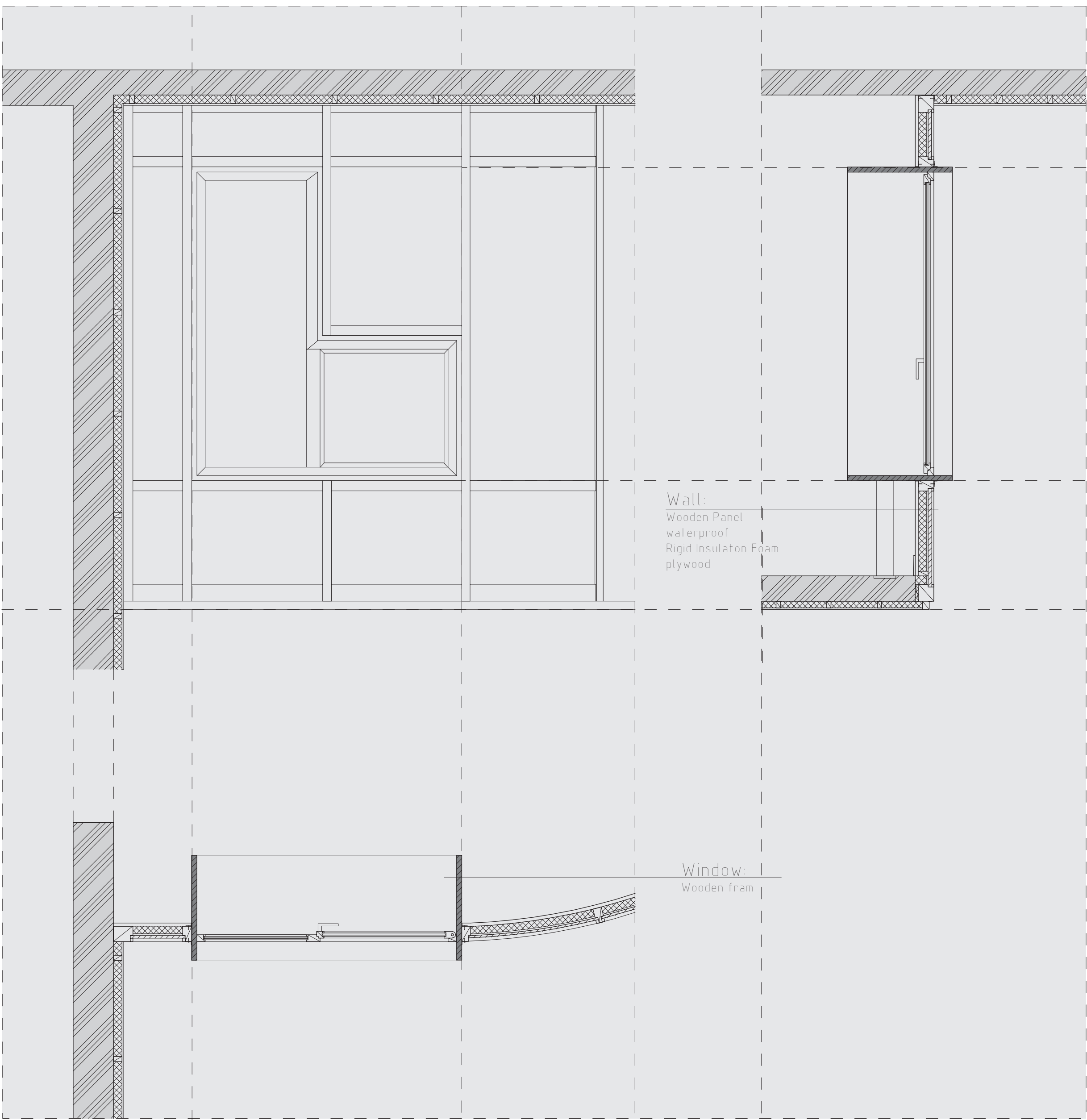
DETAIL-CORNER 5 120
